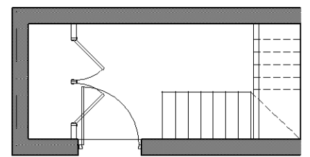
MEWS FLAT TYPE 3 (2B 4P)
