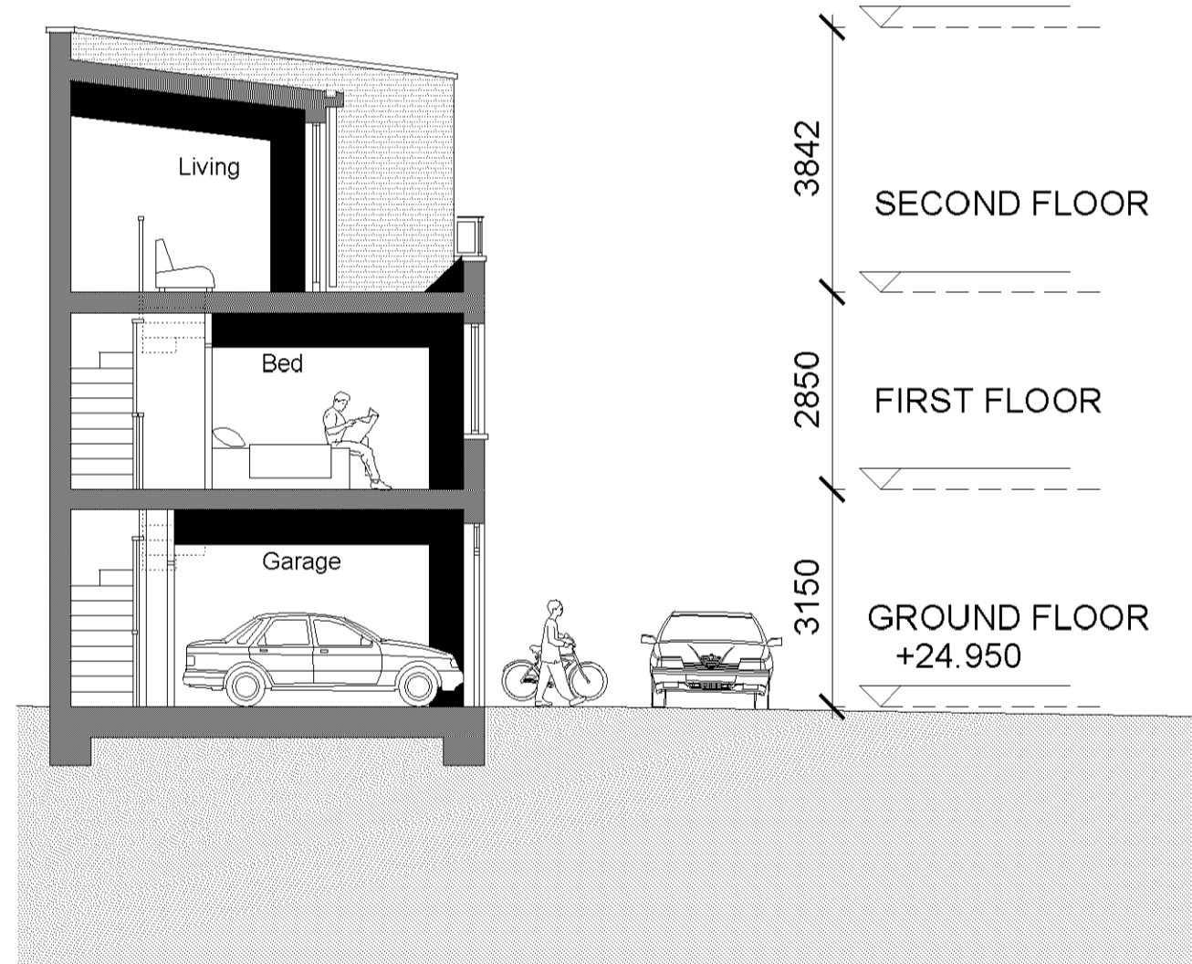
Section 1:100
