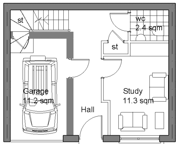
MEWS HOUSE TYPE 1 (2B 4P)
