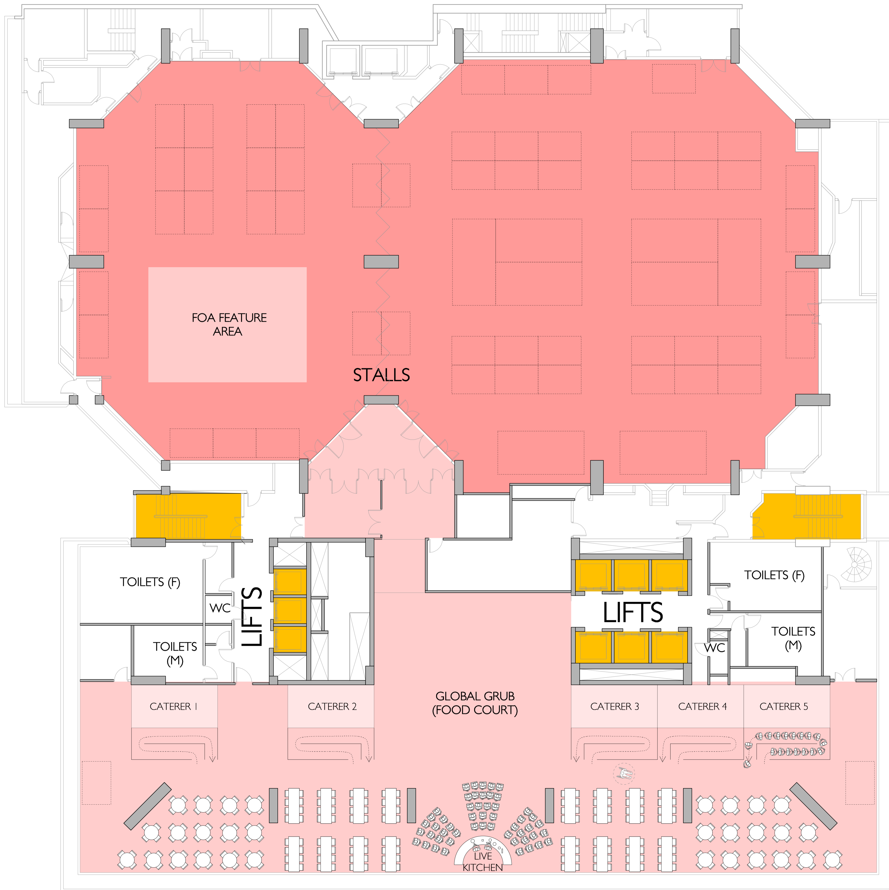
1 Third Floor Layout 1:125 @ A1
