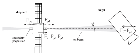
Figure 2: Schematic - Ion Beaming Concept [17]
