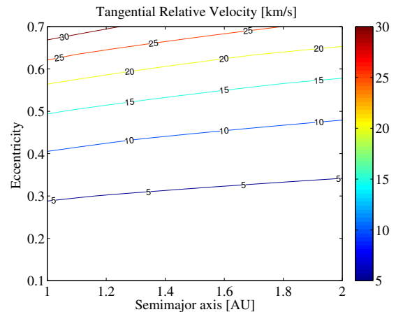
Figure 9: Achievable Relative Velocity in the Direction of the Velocity of the Asteroid
