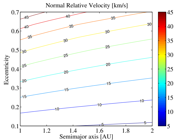
Figure 8: Achievable Relative Velocity in the Direction Normal to the Velocity of the Asteroid
