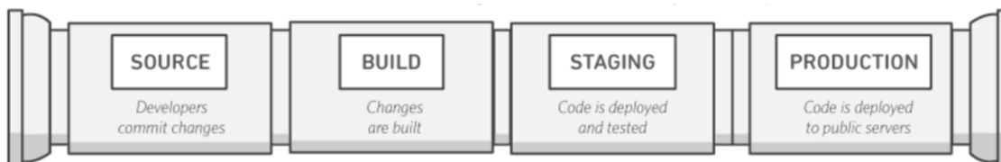
Figure 1: CI/CD pipeline
