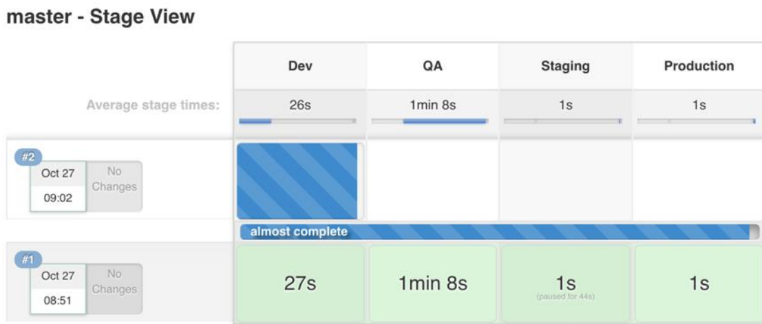
Figure 15: Defined stages of Jenkins pipeline visualized by the Pipeline Stage View Plugin
