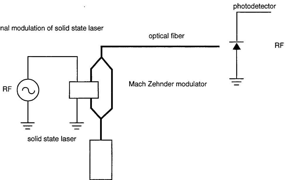
Figure 4.1 Optical Microwave Link
