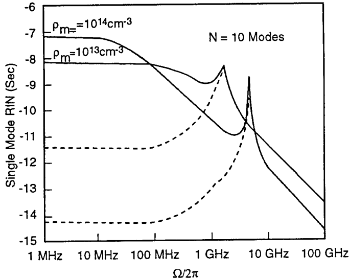
Figure 4-2. Theoretical estimates of relative intensity noise (RIN) for a single cavity mode, laser diode. At frequencies below the laser relaxation frequency the dashed lines are single mode and the solid lines are for multimode laser diodes.
