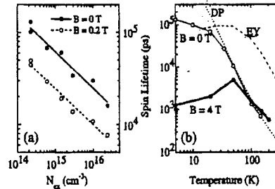
FIG. 4. (a) T_2^* vs N_{ex} . Solid lines are power-law fits to T_2^* \sim N_{ex}^{-0.4} . Data are taken at 5 K. (b) T_2^* vs temperature for n = 10^{16} at B = 0 and 4 T and N_{ex} = 2 \times 10^{16} cm^{-3} . Dotted lines are DP and EY predictions.
