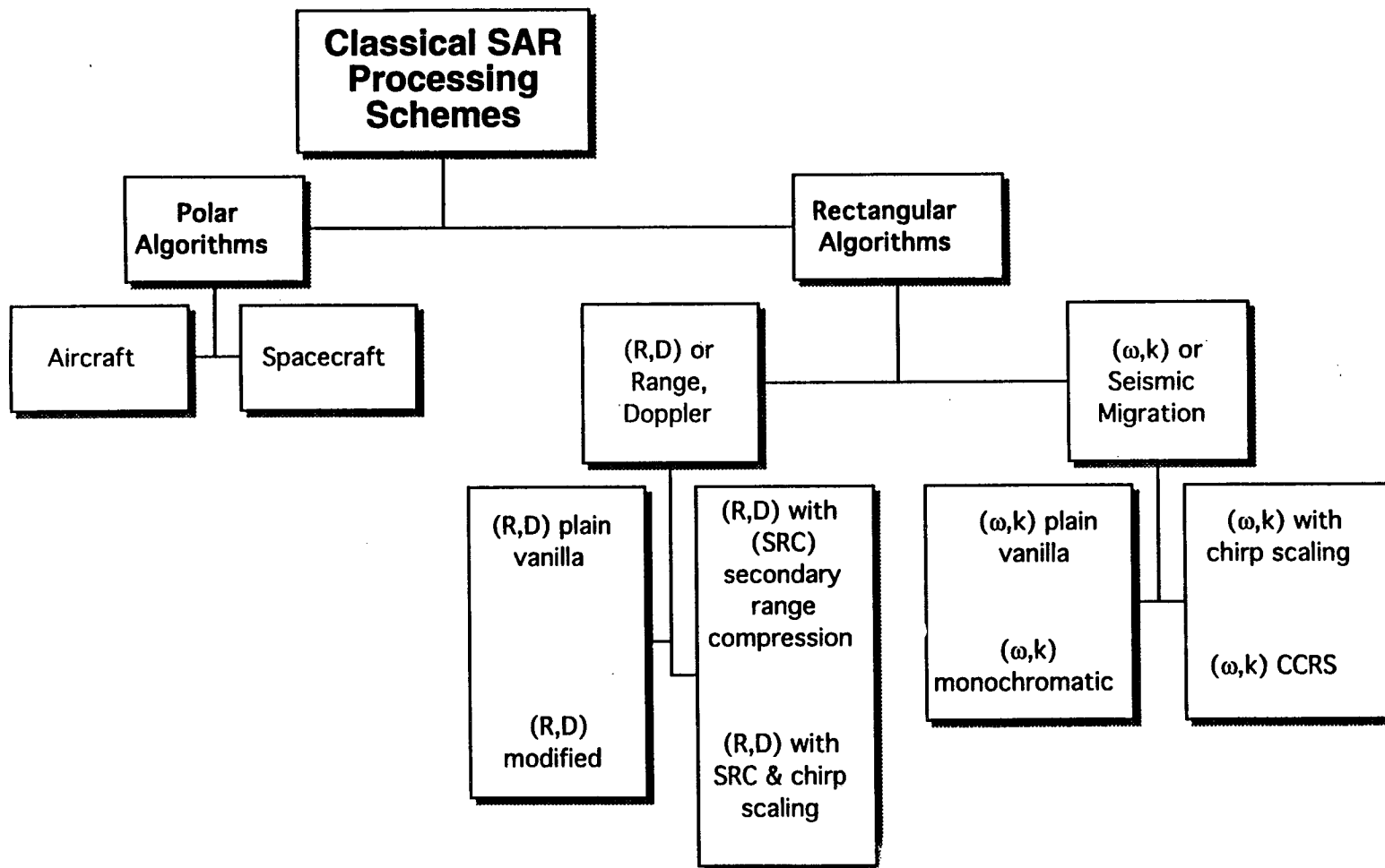
Figure 2-3. Schematic diagram of SAR Imaging Algorithms.
