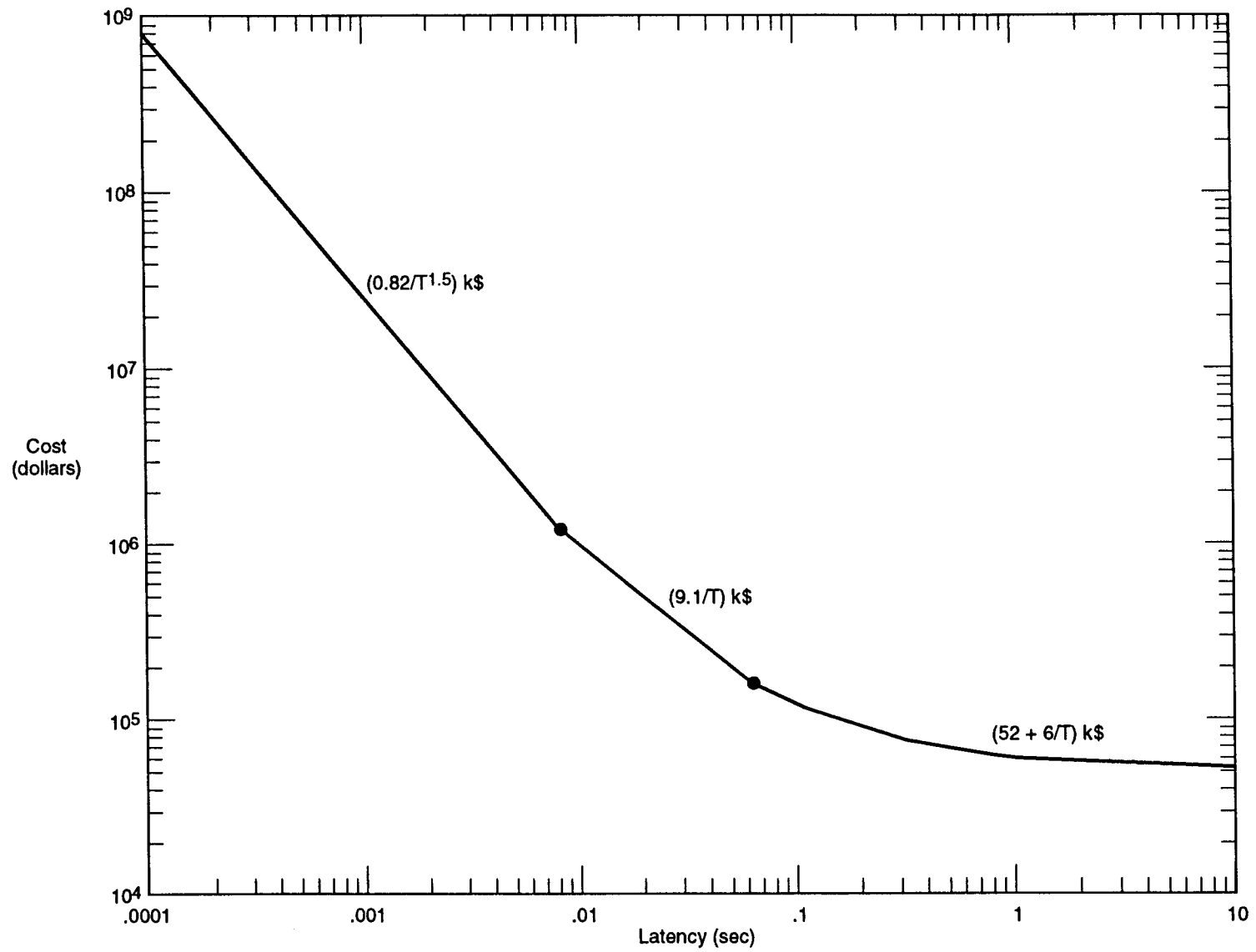
Figure 3-1. Cost as a function of latency for SAR processors implemented in 1993 technology.
