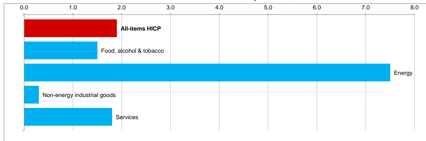
Euro area annual inflation, April 2017, %
