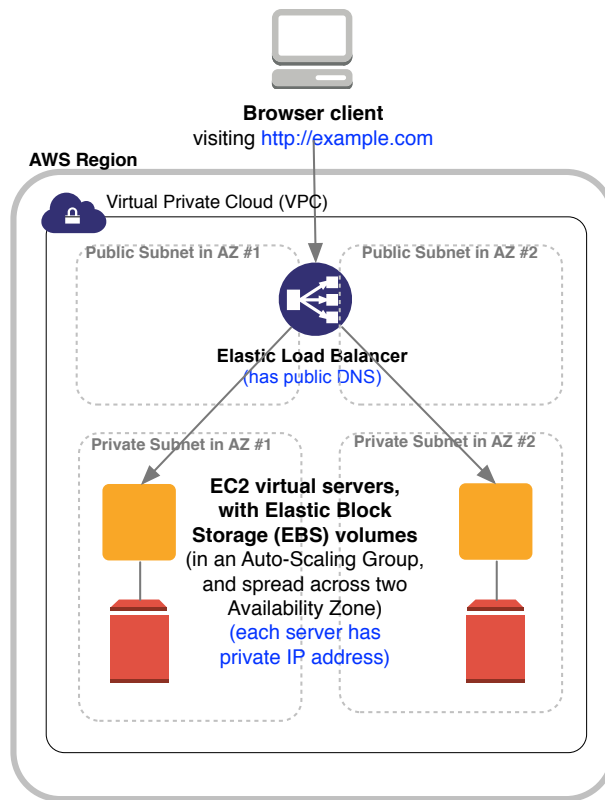
Figure 2: AWS Architecture for a “Lift and Shift”
