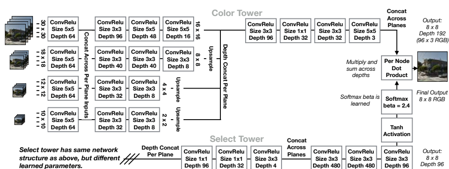
Figure 6: Full network diagram. The initial stages of both the color and selection towers are the same structure, but do not share parameters.
