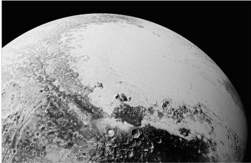
Spherical mosaic of New Horizons images (released 10 September 2015) [158][159]
