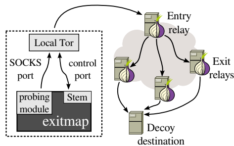
Fig. 2. The design of exitmap . Our scanner invokes a Tor process and uses the library Stem to control it. Using Stem , circuits are created “manually” and attached to decoy connections which are initiated by our probing modules.
