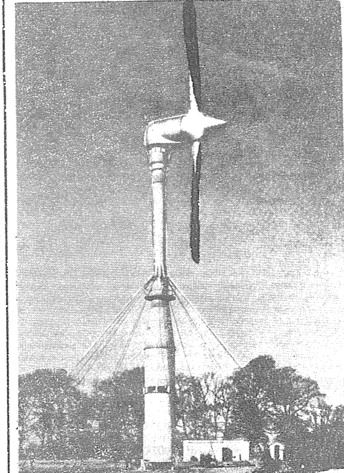
The Enfield-Andrasu wind turbine, shown above, was built in the early 1950's in England. It had a capacity of 100 Kilowatts, and a rotor of 79 feet, with hollow blades which acted as a centrifugal air pump to pull air up the hollow tower. The generator was run by an air turbine and was mounted near the ground, which is of great structural advantage.
