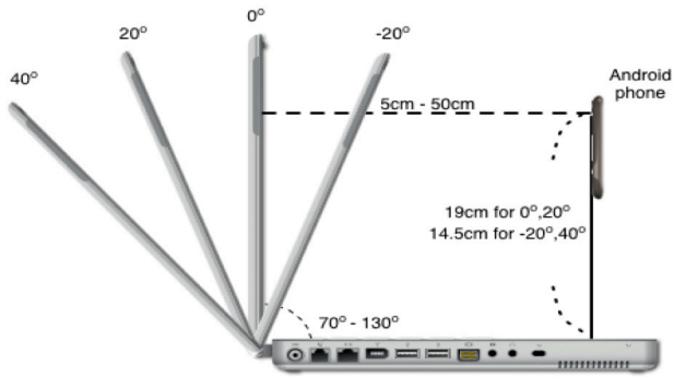
Figure 5. The setup of the reliability experiment.
