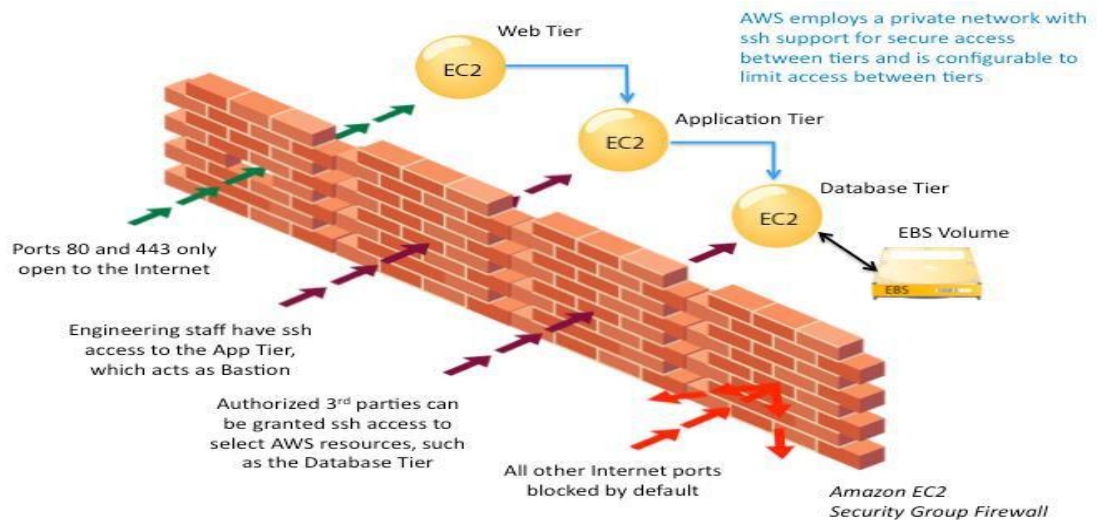
Figure 4: Amazon EC2 Security Group Firewall
