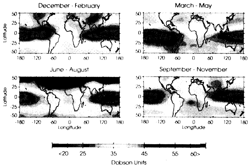
Figure 11: Observed distributions of vertical column ozone in the troposphere for 4 periods from Fishman et al. (91, 93). 1 Dobson unit represents a vertical column of 2.62 \cdot 10^{16} molecules \text{cm}^{-2} .
