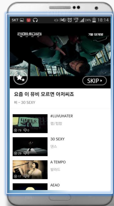
Movid
