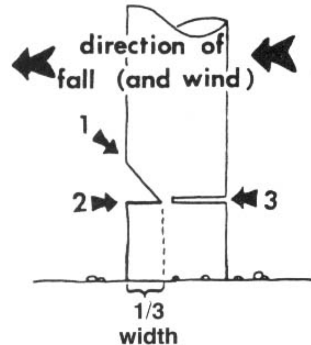
Chainsaw felling; note sequence of cuts.
