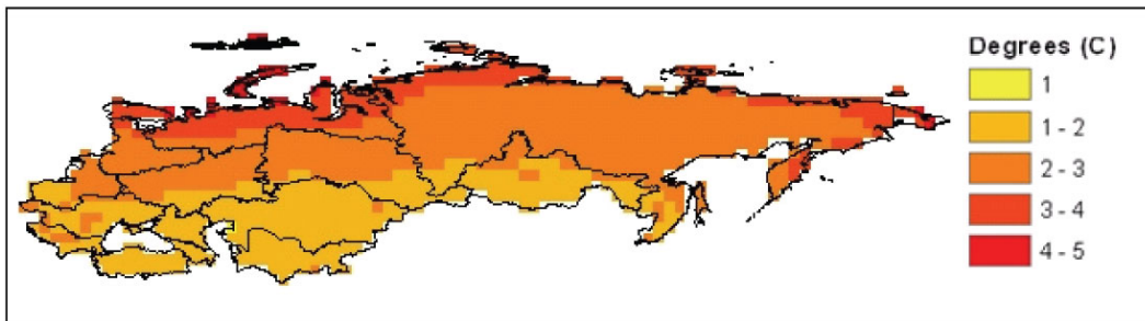
c. Change in summer (JJA) temperature (2030-2049; 1980-1999; A1B; 8 GCMs)
