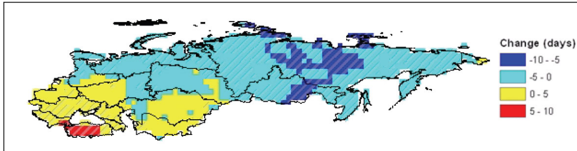
b. Change in runoff (2041-2060; 1900-1970; A1B; 8 GCMs)
