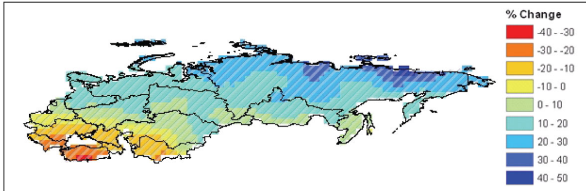
c. Change in daily rainfall intensity (2030-2049; 1980-1999; A1B; 8 GCMs)
