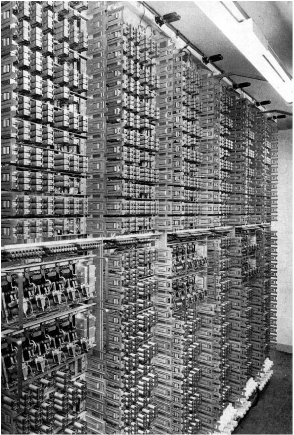
Machinery of the electrical scoreboard.
