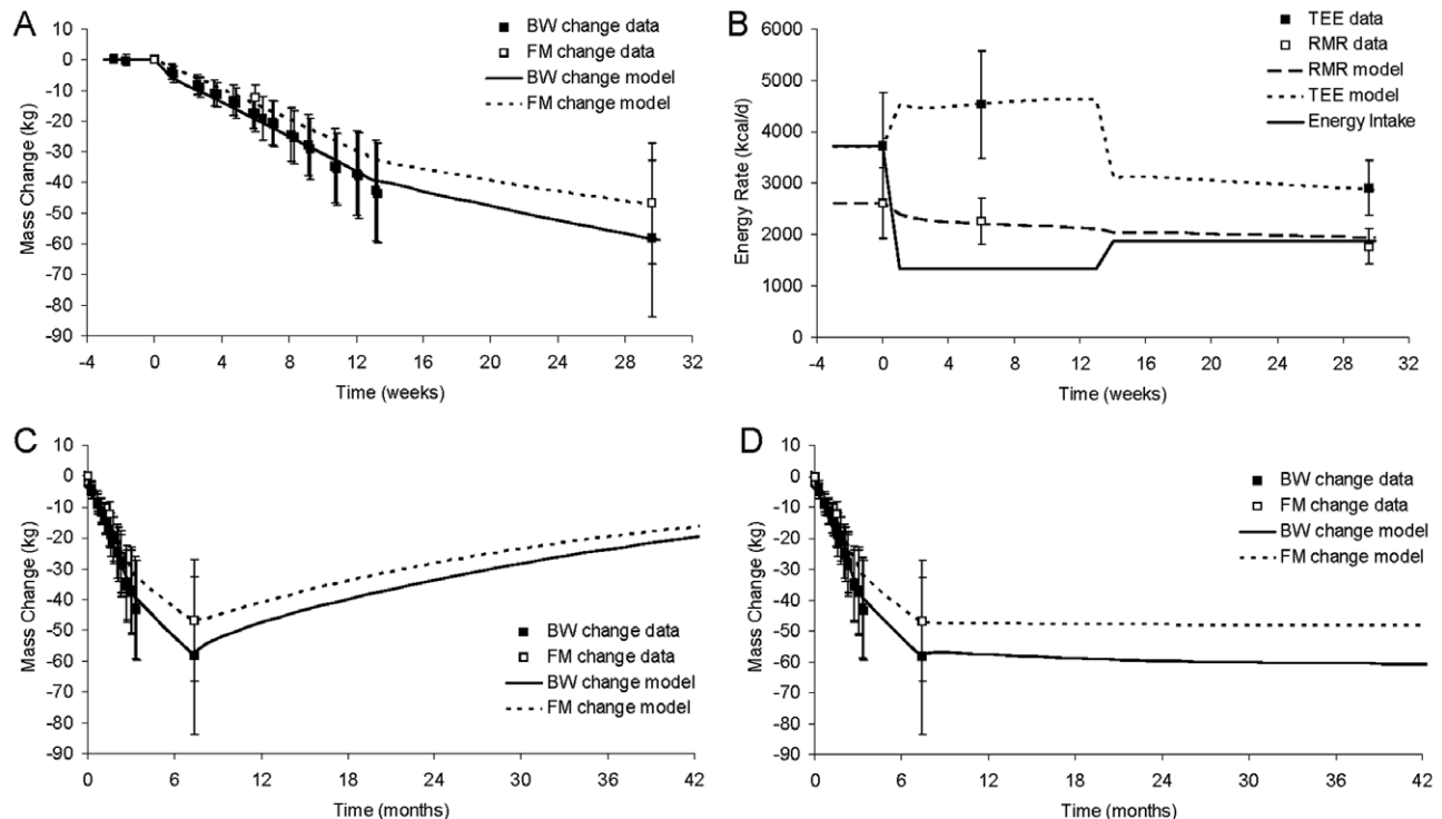
FIGURE 1 (A) Simulated (curves) and measured (boxes, mean \pm SD) BW and FM changes during The Biggest Loser competition. (B) Components of energy balance including TEE, RMR, and energy intake. (C) Slow simulated regain of BW and FM upon return to the original diet and sedentary lifestyle after 7 months. (D) Simulated maintenance of BW and FM loss with a sustained 3,000 kcal/d diet and 20 min of daily vigorous exercise after 7 months.
