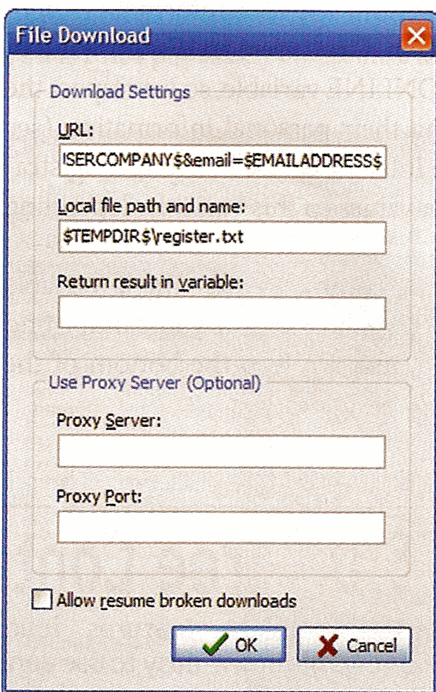
Figure 7 The File Download Plug-In
