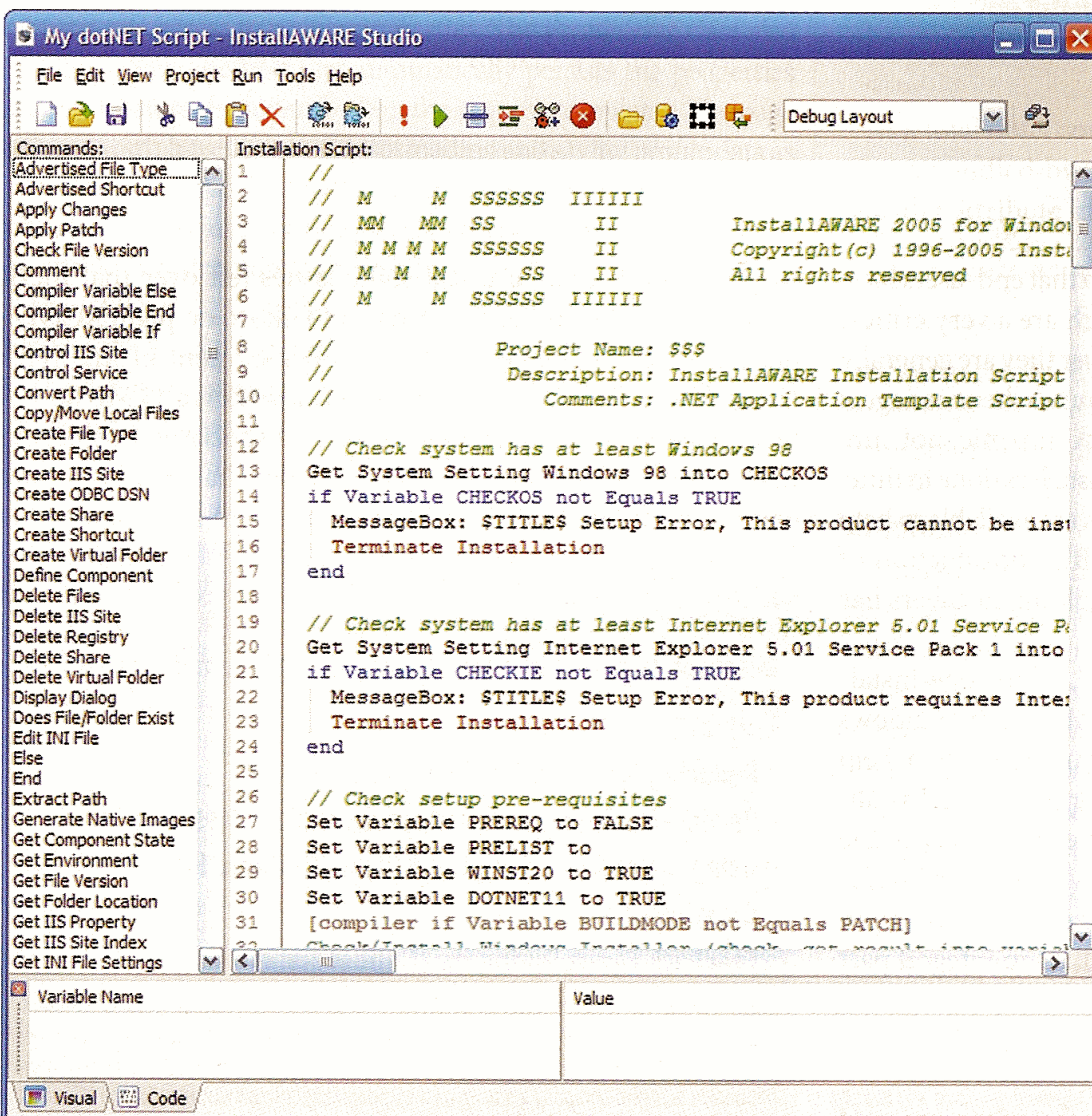
Figure 2 The InstallAware Script
