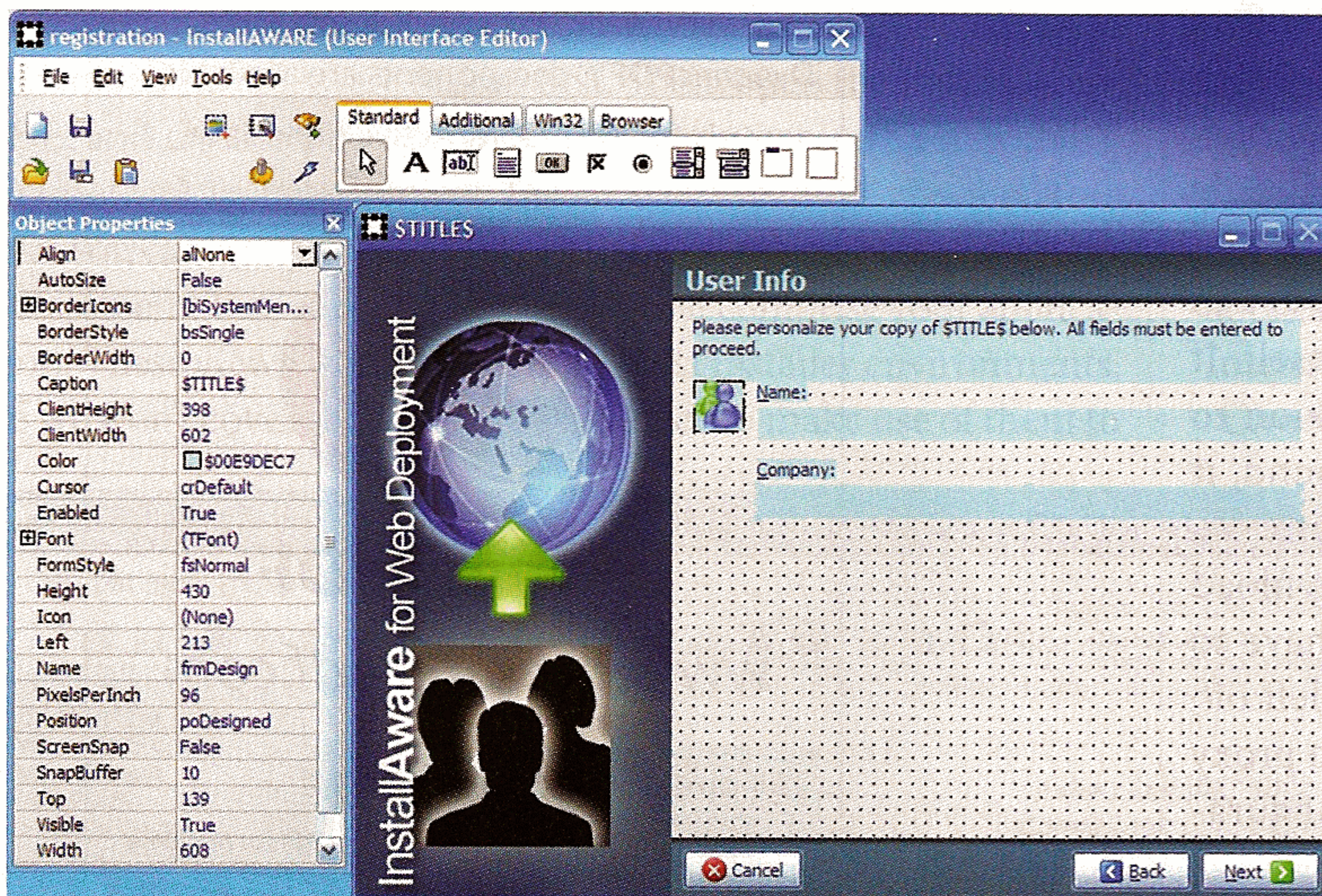
Figure 3 The Dialog Editor
