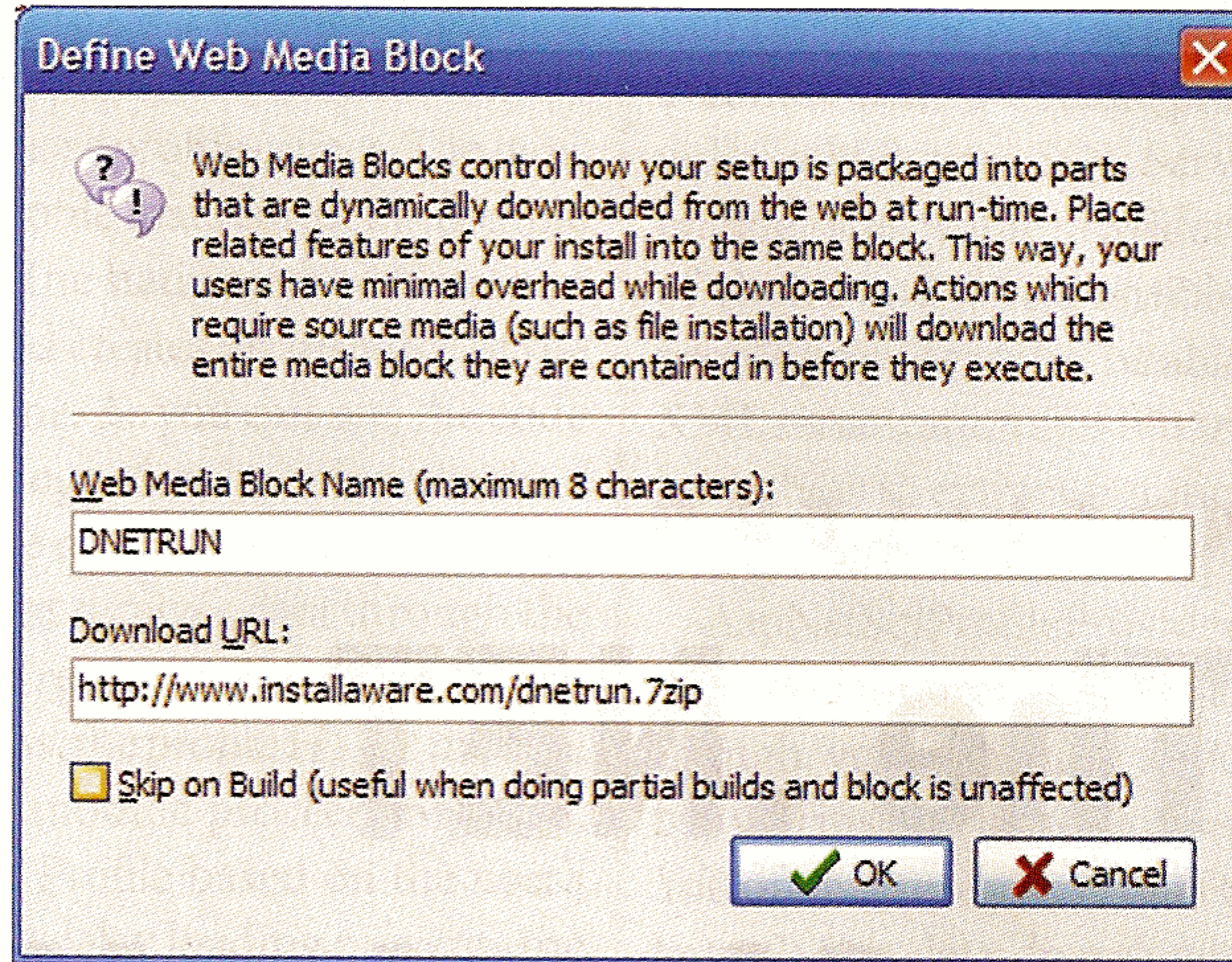
Figure 1 Defining a Web Media Block
