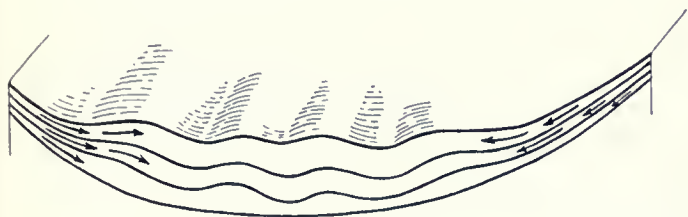
Crumpling produced by compressive settling into a depositional basin from the higher margins. Length of section may be up to 75 miles.
