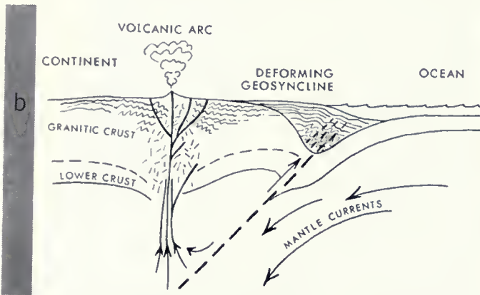
a) geosyncline developing; granite forming and volcanism in adjacent belt; b) geosyncline deforming; c) uplift, metamorphism and granite formation as mantle currents wane.
