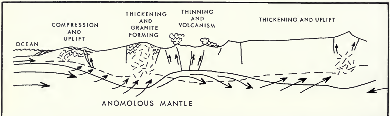
Possible effects of 'thinning' and 'thickening' of the crust from below by the action of currents in the upper mantle: the broken line represents the earlier base of the crust, the lower continuous line the modified base.
