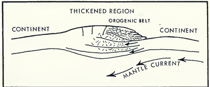
Below: Thickening of crust by underthrusting of one continent by another under the influence of mantle currents; thickening may also be caused by compression.
