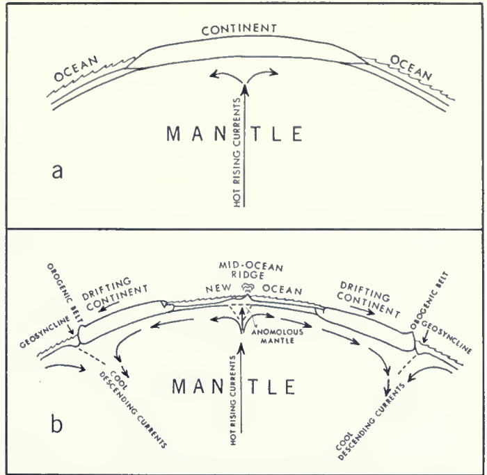
Above: Shows continental drift, mid-ocean ridges, and compressional orogenic belts resulting from convection currents in the mantle; a) initial stage of currents ascending beneath continent; b) mature stage, continents drifting and new ocean formed.
