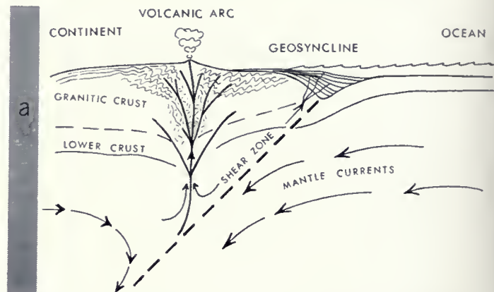
Diagrammatic vertical sections across a developing orogenic belt assuming of convection currents in the mantle as the driving mechanism:
