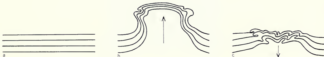
A possible effect of uplift followed by subsidence: (a) a series of horizontal strata; (b) uplift with consequent stretching and thinning of the beds (c) subsidence with folding of the stretched beds.
