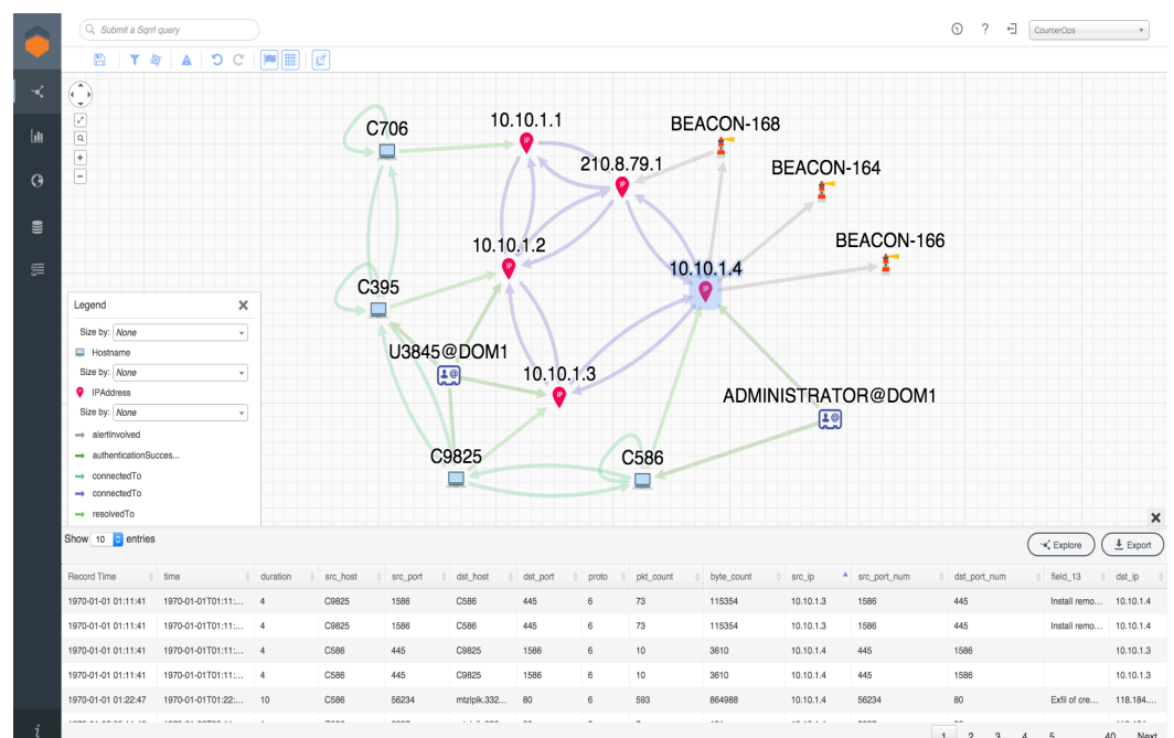
The Sqrll UI, featuring the Behavior Graph and data exploration
