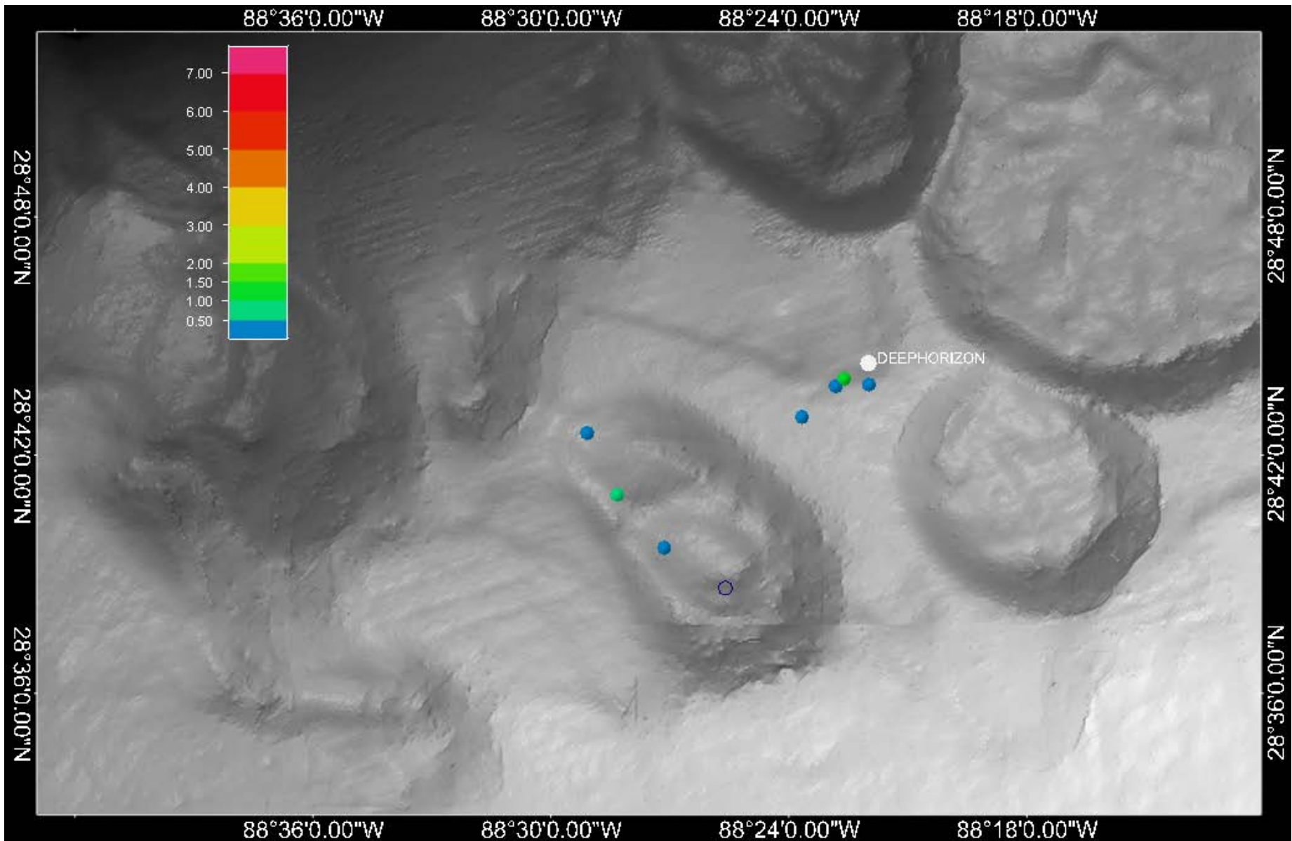
Figure 13: Mean Fluorescence ppb (QSDE) between 1000-1300m on 20 May 2010
