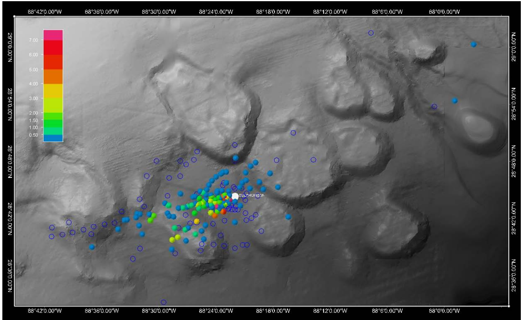
Figure 45: Mean Fluorescence ppb (QSDE) between 1000-1300m from 19 May through 19 June – with far field R/V Gordon Gunter stations
