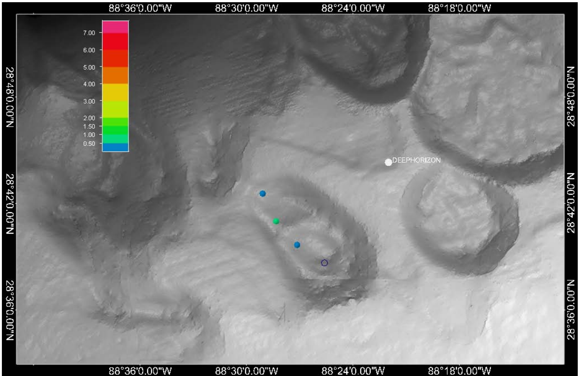
Figure 12: Mean Fluorescence ppb (QSDE) between 1000-1300m on 19 May 2010
