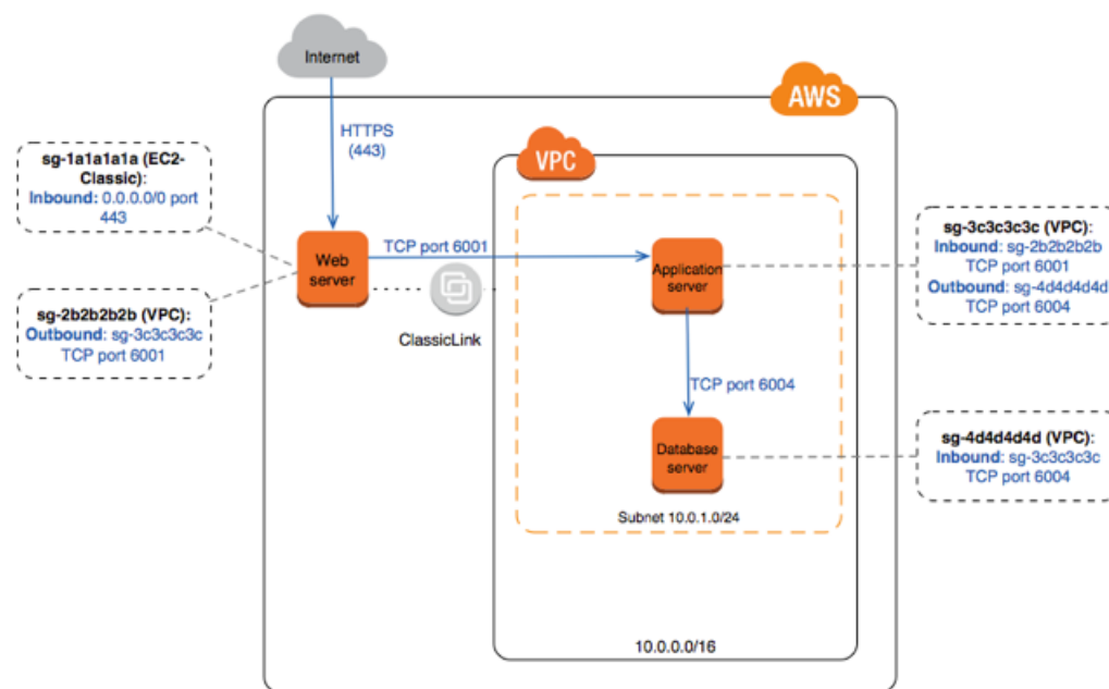
Security Groups for Your Web Server ( sg-1a1a1a1a and sg-2b2b2b2b )
