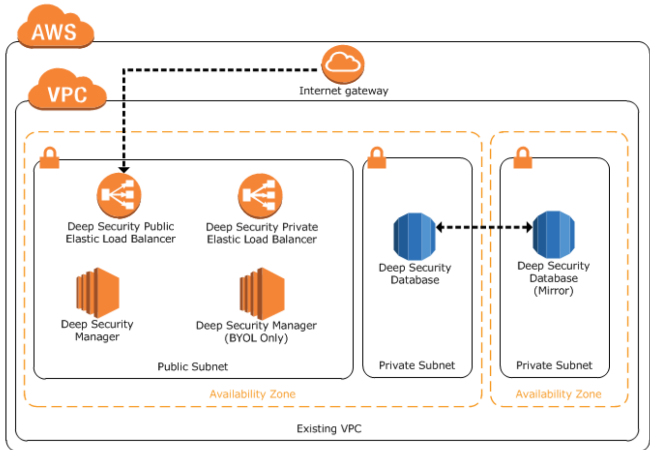
Figure 1: Trend Micro Deep Security Architecture on AWS
