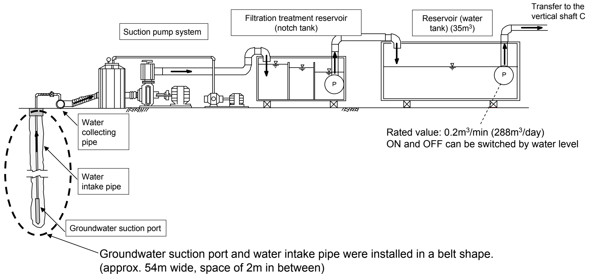
Well point plant
