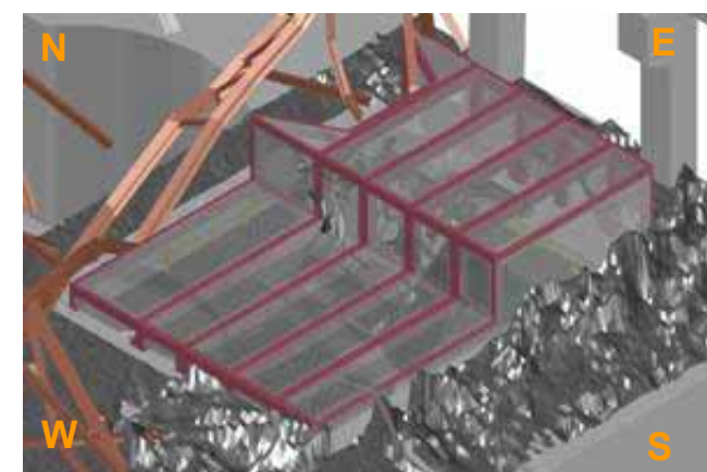
Simulated image of the protection installed on the spent fuel pool (first phase)
