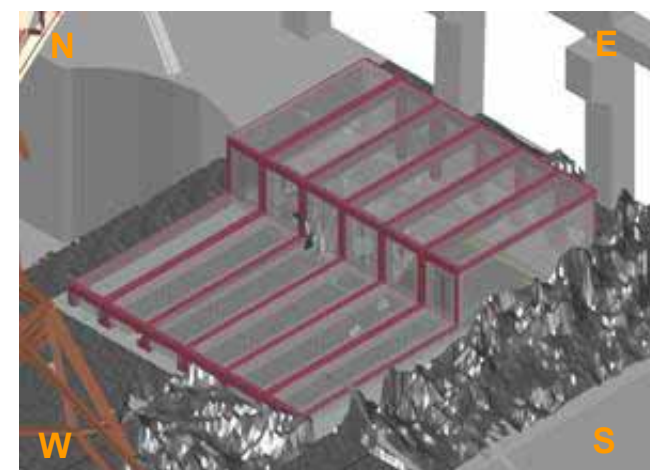
Simulated image of the protection to be installed on the spent fuel pool (second phase)
