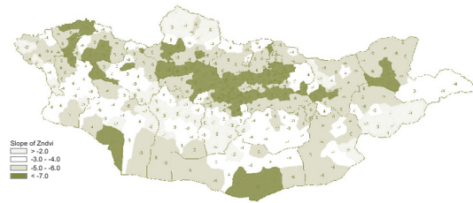
Figure 3.10: Slope of Z Normalized Difference Vegetation Index (ZNDVI), Mongolia, 2007
