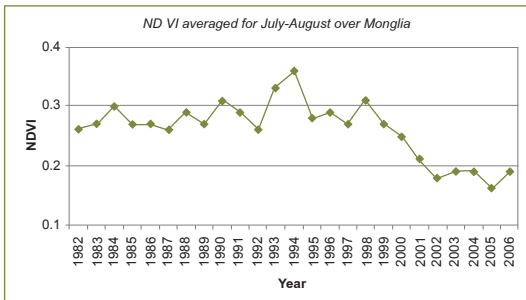
Figure 3.9: Normalised difference vegetation index (NDVI) for July and August, Mongolia, 1982-2006
