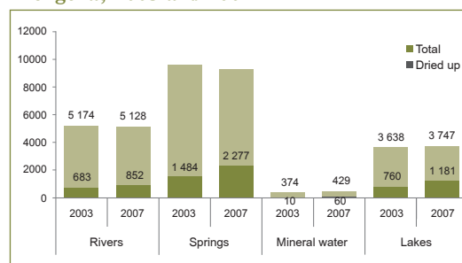
Figure 2.1: Surface water sources drying up, Mongolia, 2003 and 2007
