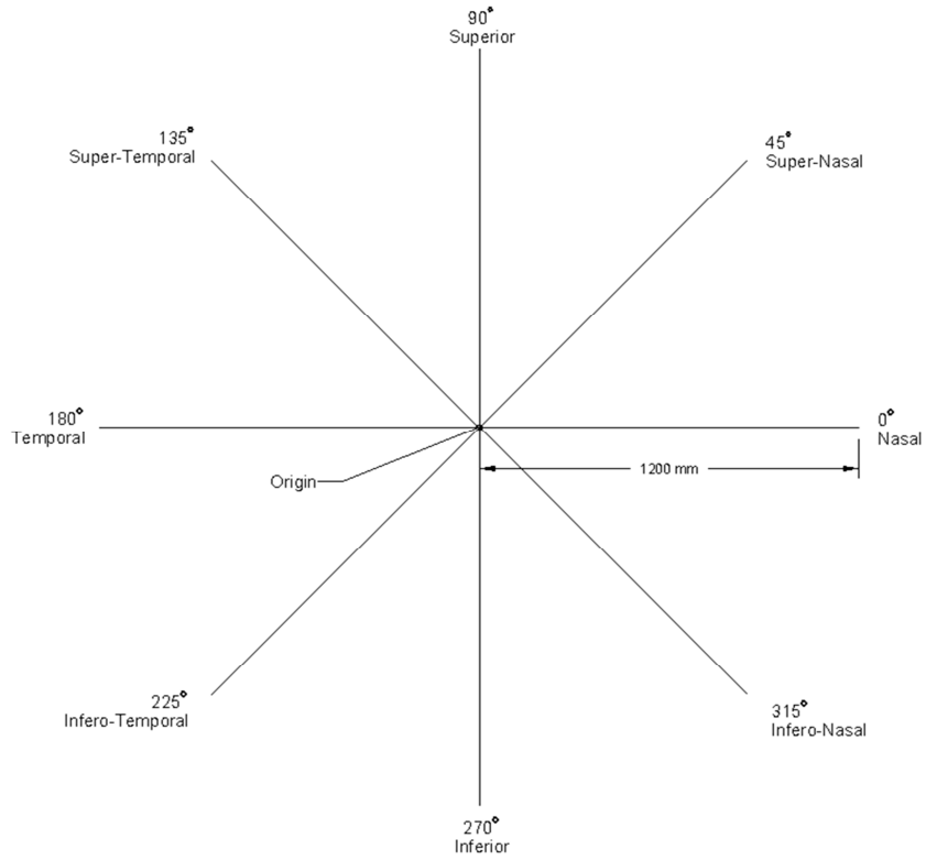
Figure 1. Static FOV Axes (Oriented to the left pupil of the head form)
