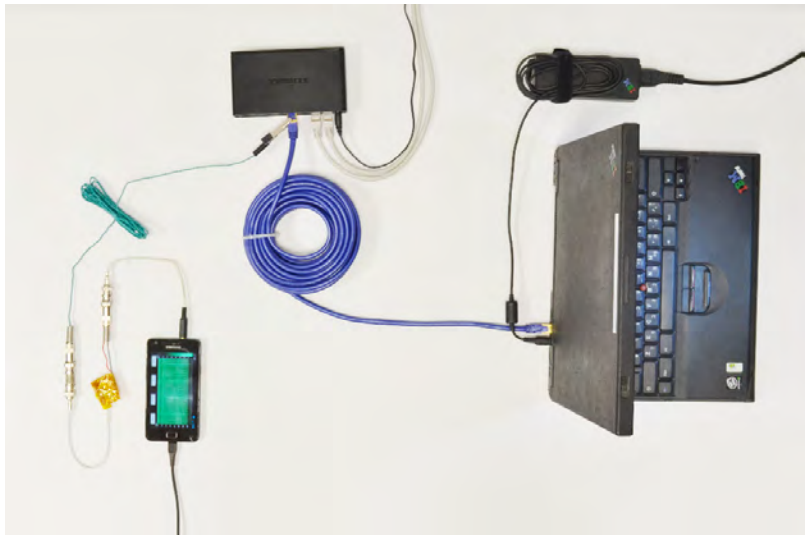
(b) Adaptive “far end of cable” attack using a mobile phone. The chassis potential of the laptop is measured from the far side of an Ethernet cable (blue, 10 m long). An alligator clip connected to a plain wire (green) taps the shield of the Ethernet cable where it connects to an Ethernet switch. The signal passes through a passive filter (orange) and then, via a coax cable (white), into the microphone/earphone jack of the phone (Samsung Galaxy S II), where it is amplified and digitized. The phone itself is grounded to mains earth via its USB port. It is possible to perform the adaptive attack using this setup.
