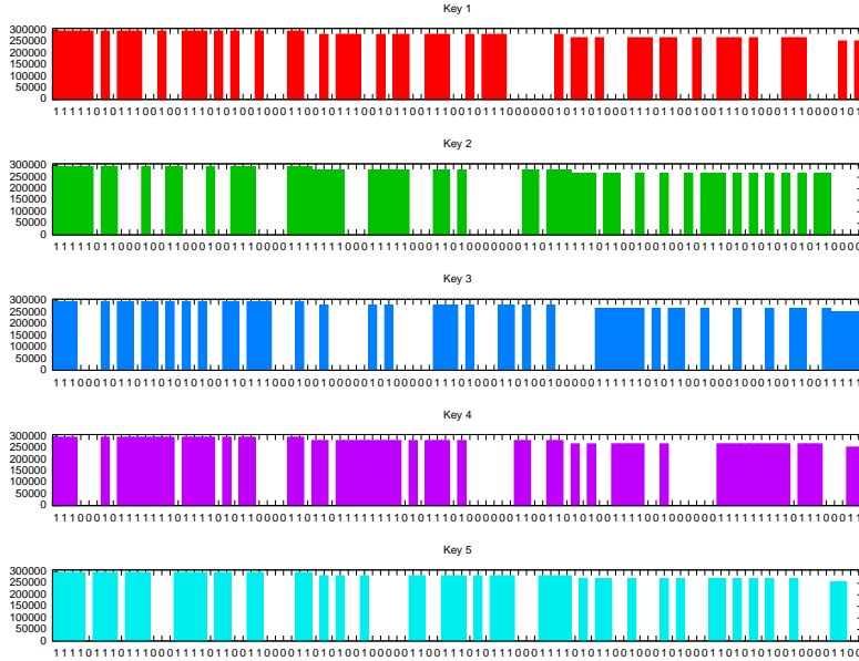
Figure 7: Number of zero limbs in the second operand of \text{MUL\_BASECASE}(a, b) during an execution of the modular exponentiation routine with the secret prime p using our attack and randomly generated keys. The correct bit values are indicated on the horizontal axis of each key.
