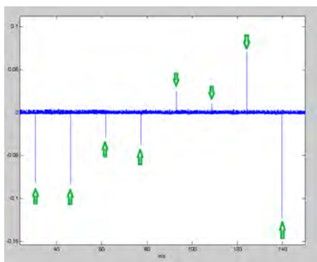
Figure 10: Frequency demodulation of the leakage signal during a decryption operation using a randomly generated 4096-bit RSA key. The interrupts, occurring every 15 milliseconds, are marked by green arrows.
