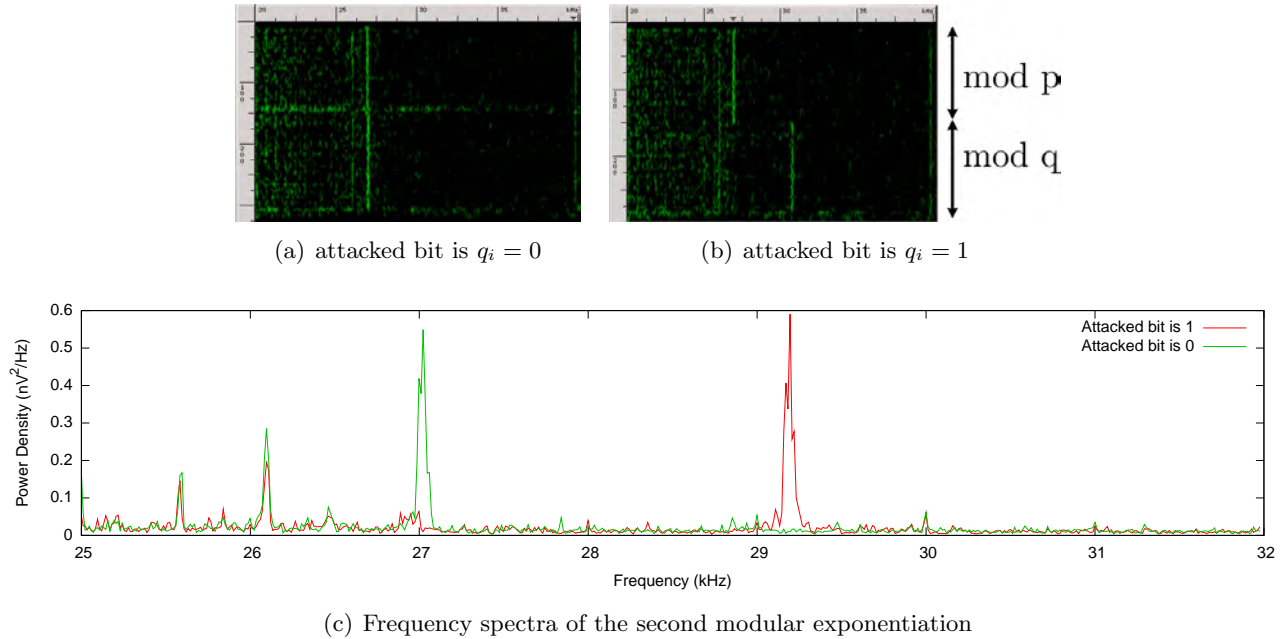
Figure 11: Chassis measurement of RSA decryption for various values of the attacked bit executed on a Lenovo ThinkPad T60.
