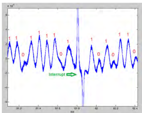
Figure 9: Frequency demodulation of a segment of the leakage signal obtained during a decryption operation using a randomly generated 4096-bit RSA key. Note the correlation between the signal and the secret key bits.
