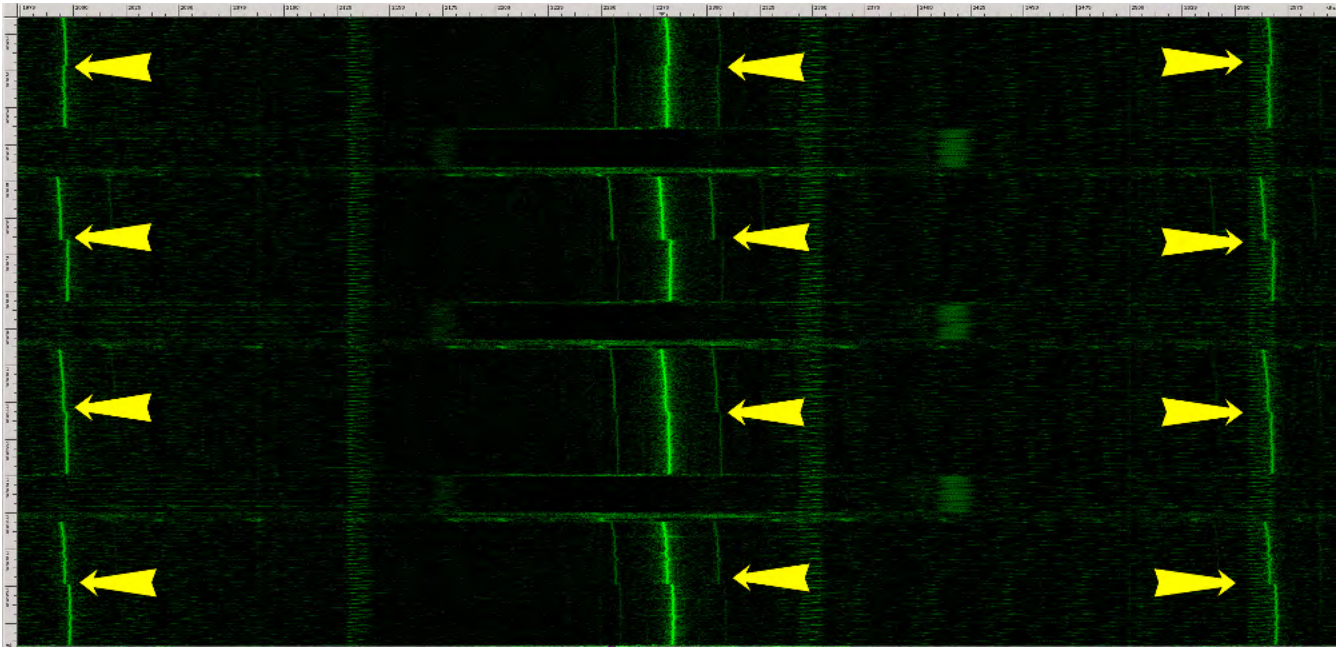
Figure 4: Chassis measurement (1.7 sec, 1.9–2.6 MHz) of four GnuPG RSA signatures executed on a Lenovo 3000 N200. The transitions between p and q are marked with yellow arrows.
