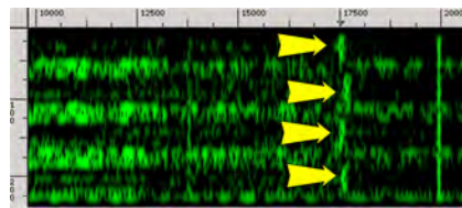
Figure 5: Chassis measurement (0.20 sec 0–20 kHz) of four ElGamal decryptions using the same message and randomly generated 3072 bit keys executed on a Lenovo ThinkPad T61.
