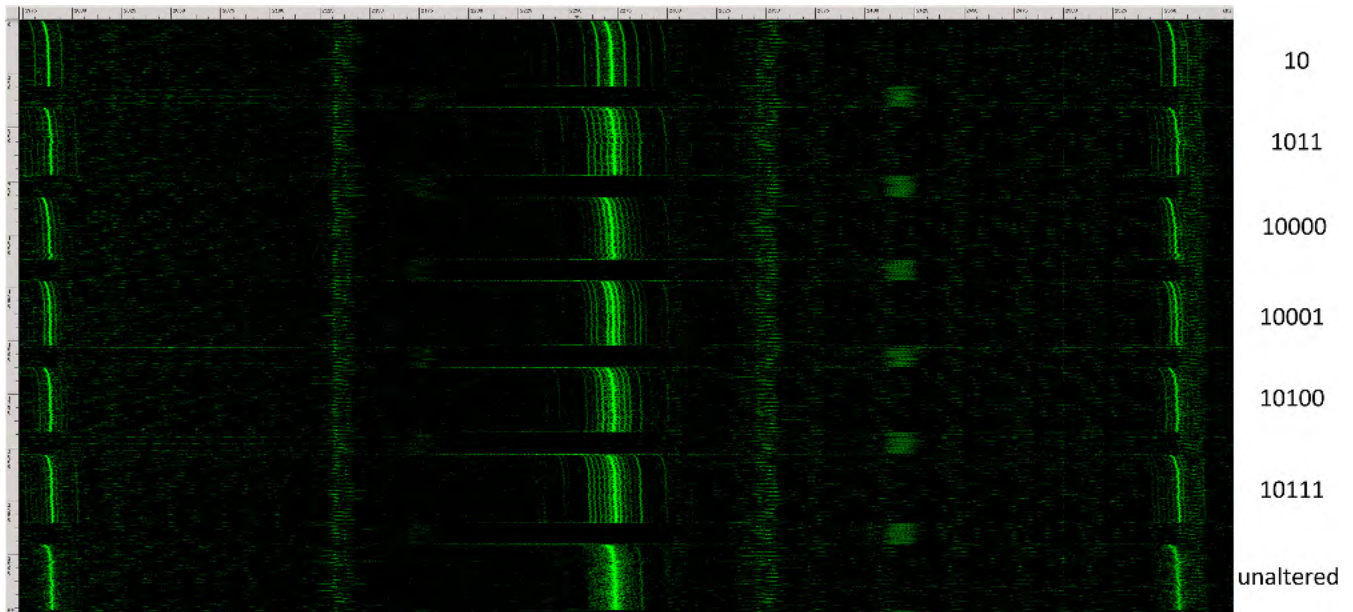
Figure 8: Chassis measurement (2.5 sec, 1.9–2.6 MHz) of seven GnuPG RSA decryptions executed on a Lenovo 3000 N200 laptop. In the first 6 cases, exponents ( d_p and d_q ) are both overridden to be the 2048-bit number obtained by repeating the pattern written to the right. In the last case, the exponent are unaltered. In all cases, the moduli p and q are the same and the ciphertext is set to n - 1 .
