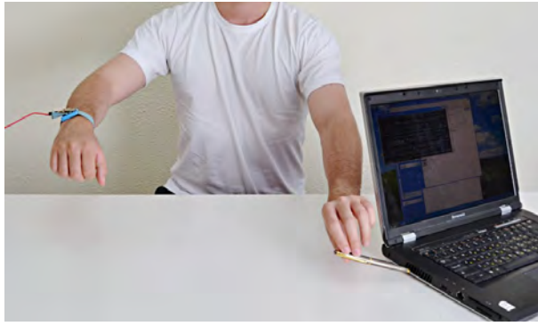
(a) Non-adaptive “human touch” attack through a metal pen touching the heatsink fins. The wristband is connected to the probe wire.
