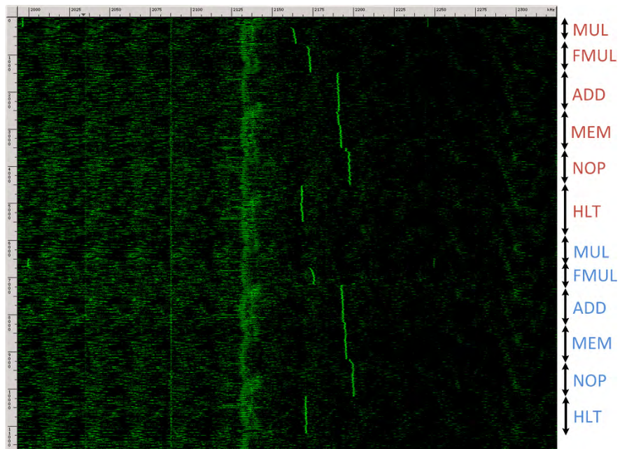
Figure 3: Frequency spectrogram (1.1 sec, 2-2.3 MHz) of a recording of different CPU operations obtained while measuring the attacker's body potential while touching an exposed part of the chassis of a Lenovo 3000 N200 laptop.
