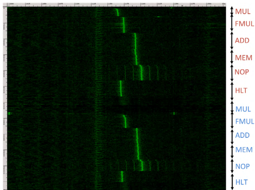
Figure 1: Frequency spectrogram of the chassis potential, while running different CPU operations using a Lenovo 3000 N200 laptop. The horizontal axis is frequency (2–2.3 MHz), the vertical axis is time (10 sec), and intensity is proportional to the instantaneous energy in that frequency band.
