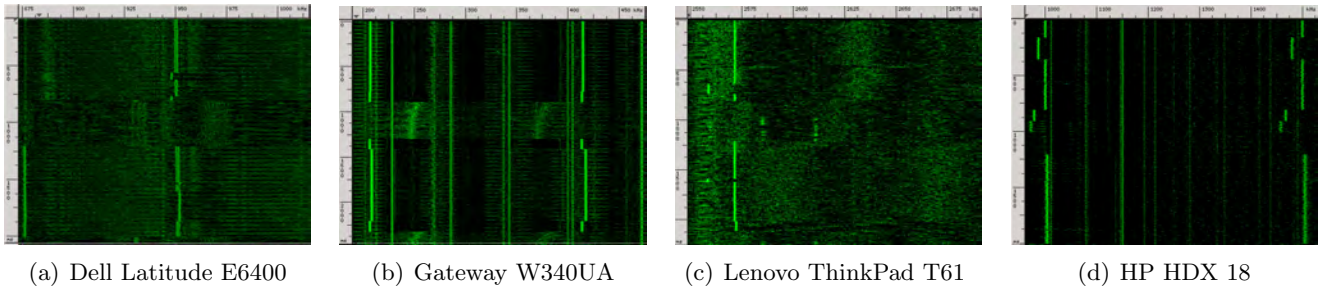
Figure 2: Chassis measurements of various target computers performing MUL, HLT and MEM in this order. Note that the three operations can be distinguished on all machines.
