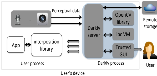
Figure 1. System architecture of DARKLY.
