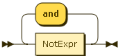
Figure 5.23. AndExpr
