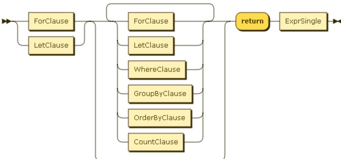
Figure 5.36. FLWORExpr
