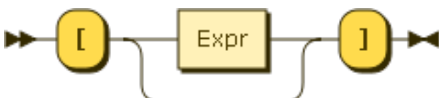
Figure 5.11. ArrayConstructor
