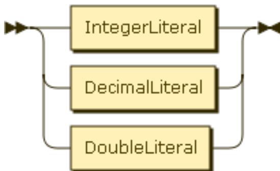
Figure 5.2. NumericLiteral
