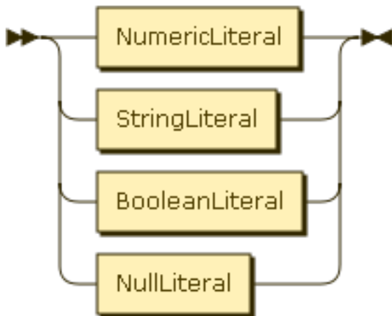
Figure 5.1. Literal
