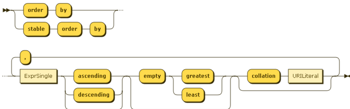
Figure 5.39. OrderByClause
