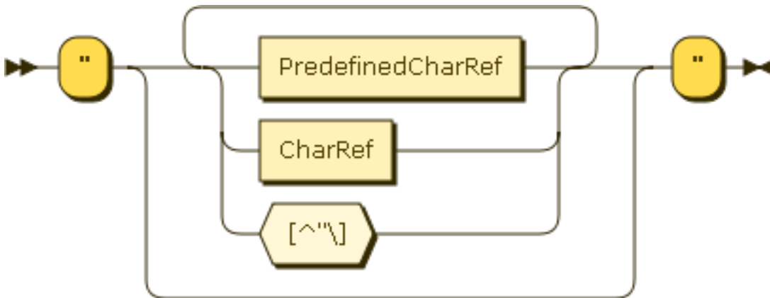
Figure 5.6. StringLiteral
