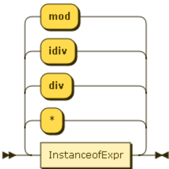
Figure 5.17. MultiplicativeExpr
