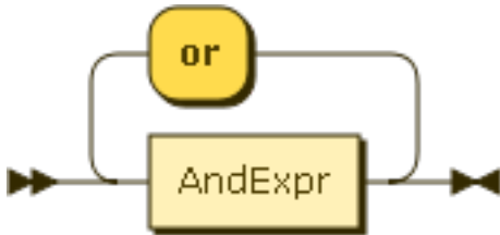
Figure 5.22. OrExpr
