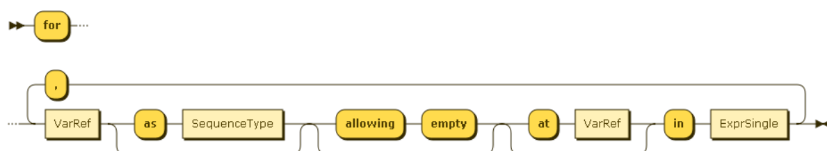
Figure 5.37. ForClause
