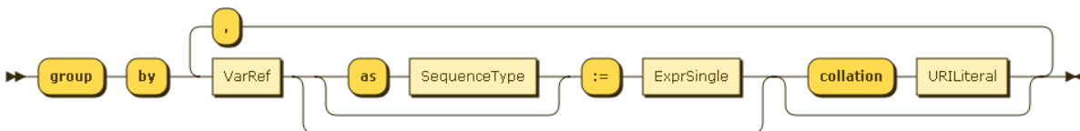
Figure 5.40. GroupByClause
