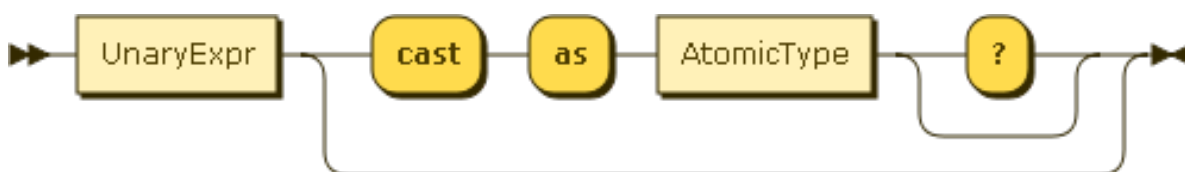
Figure 5.50. CastExpr
