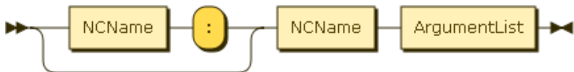
Figure 5.26. FunctionCall
