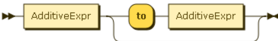
Figure 5.14. RangeExpr
