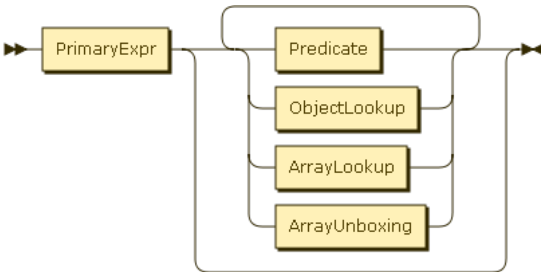
Figure 5.27. PostfixExpr
