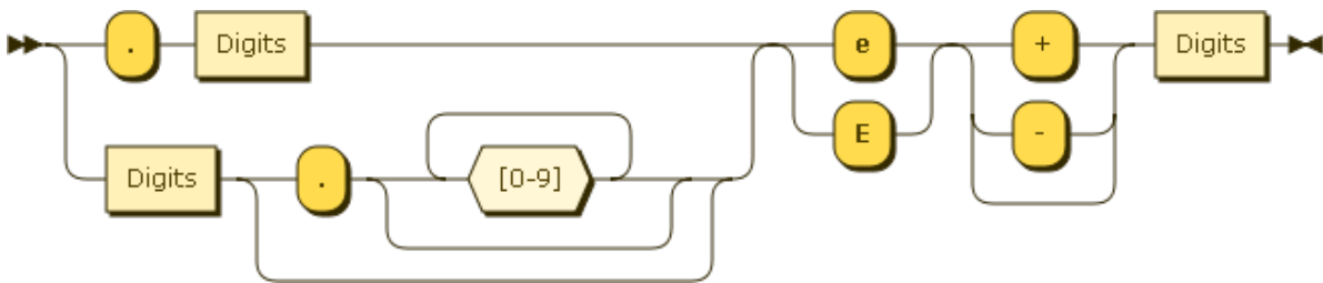
Figure 5.5. DoubleLiteral
