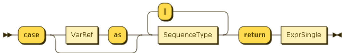
Figure 5.52. CaseClause
