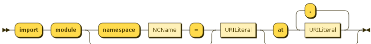
Figure 7.5. ModuleImport
