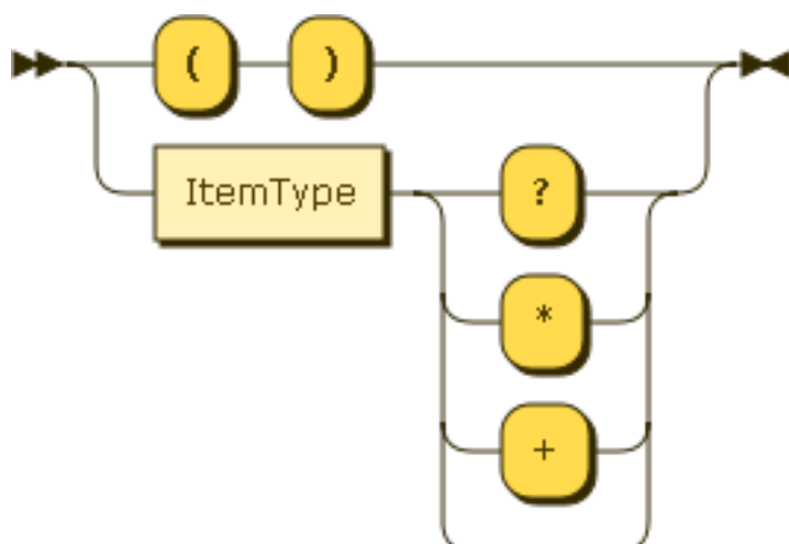
Figure 4.4. SequenceType
