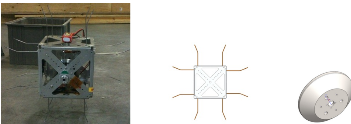
Figure 18: Prototype and CAD models (not to scale). The prototype, without the flywheel, has a mass of 1.39 kg and a moment of inertia about the axis of rotation of \approx 0.054 \text{ kg m}^2 . The flywheel is 0.57 kg and 8.07 \times 10^{-4} \text{ kg m}^2 .
