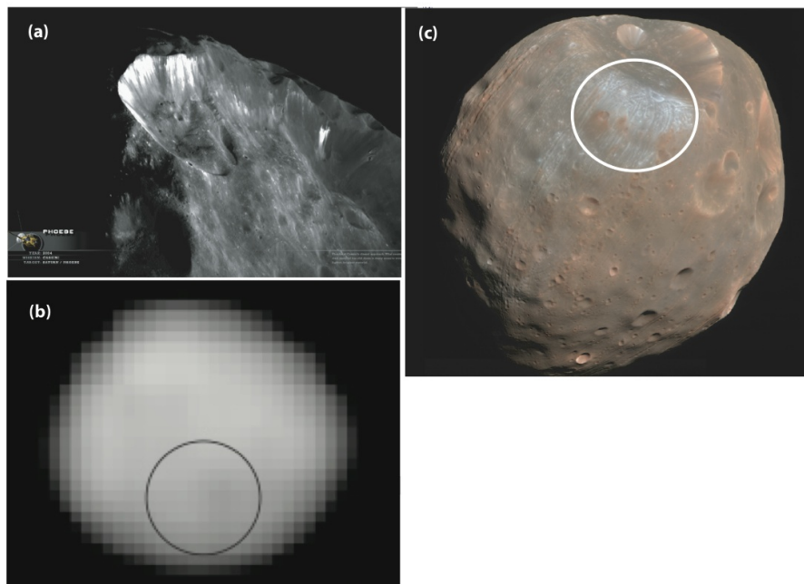
Figure 9: These pictures capture the chemical and physical diversity observed at asteroids and irregular satellites. (a) North pole of Saturn’s satellite Phoebe obtained by the Cassini-Huygens mission; while the satellite’s albedo is less than 0.1, high-albedo material can be seen on crater walls, which suggests that the dust cover is only a few tens of meter thick (Credit: NASA/ISS/CICLOPS). (b) Pallas’ surface as seen by the Hubble Space telescope [24]; the circle indicates a low-albedo area associated with a large impact basin. (c) Phobos by HiRISE on the Mars Reconnaissance Orbiter; lateral variations in color properties suggest that Phobos’ material has different origins (Credit: NASA/University of Arizona).
