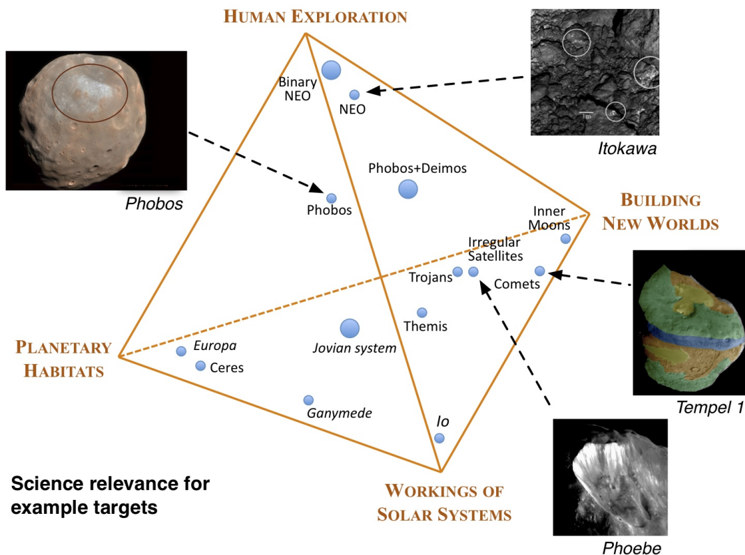
Figure 8: Relevance of different small bodies with respect to both the three themes of the decadal survey report and the vision for future human exploration (the four themes are represented as corners of the polygon). The position of a target within the polygon represents its relative relevance. For example, comets are expected to be among the most primitive objects in the Solar System although space observations indicate that they also exhibit a large variety of landscapes that result from long-term geological activity; hence, their position is in between two corners of the polygon. Another example is Phobos whose surface exploration would pertain to all four themes, as detailed in this report. The exploration of several components of a multinary system is expected to increase the overall science return of a mission, which is symbolized by bigger circles.
