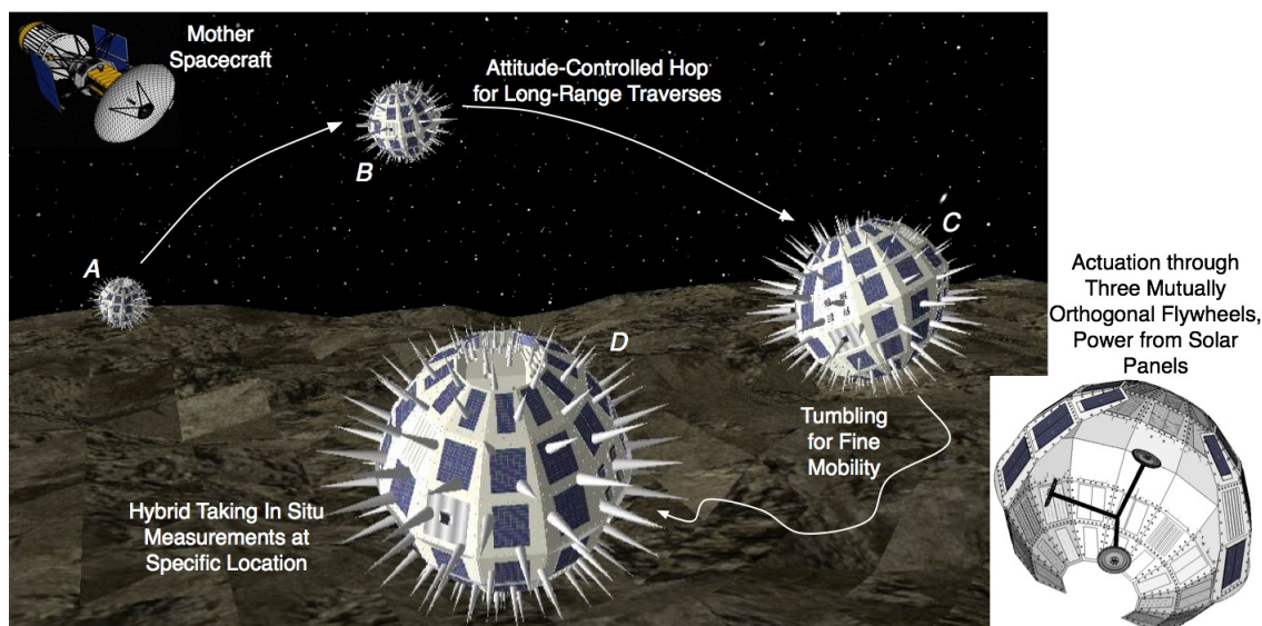
Figure 6: The mission architecture: one mother spacecraft would deploy on the surface of a small body one (or more) spacecraft/rover hybrids (from dm- to m-scale). Once deployed, the hybrids would perform attitude-controlled hops for long-range traverses (on the order of 10 m per hop, steps A to B to C in the figure) and would tumble to reach specific locations (steps C to D in the figure). Each hybrid is sealed in one enclosure and internally actuated through three mutually orthogonal flywheels (see bottom-right figure). Synergistic mission operations would ensure precise planning and control of the hybrids, while keeping their end-to-end design minimalistic.
