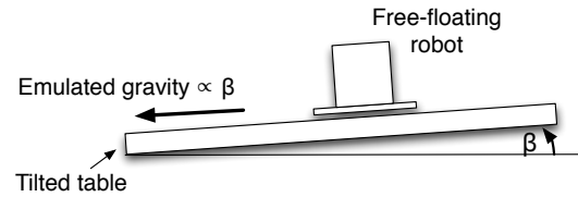
Figure 4: 3 DOF test stand on a frictionless table; by tilting the granite table, one can create a “small” force that emulates a low gravity field.
