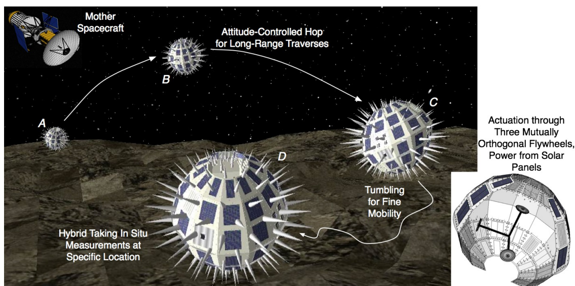
Figure 1: The mission architecture: one mother spacecraft would deploy on the surface of a small body one (or more) spacecraft/rover hybrids (from dm- to m-scale). Once deployed, the hybrids would perform attitude-controlled hops for long-range traverses (on the order of 10 m per hop, steps A to B to C in the figure) and would tumble to reach specific locations (steps C to D in the figure). Each hybrid is sealed in one enclosure and internally actuated through three mutually orthogonal flywheels (see bottom-right figure). Synergistic mission operations would ensure precise planning and control of the hybrids, while keeping their end-to-end design minimalistic.
