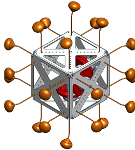
Figure 19: Second prototype of the hybrid. Note the lily-petal design of the tips of the spikes.
