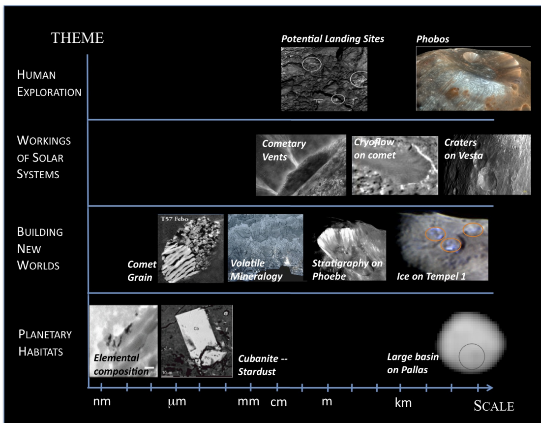
Figure 7: Illustration of the type of observations needed in order to successfully address the three cross-cutting themes highlighted in Vision and Voyages . Note that in general we lack high-resolution observations at the mm to the meter scale that could be best obtained by in-situ exploration.
