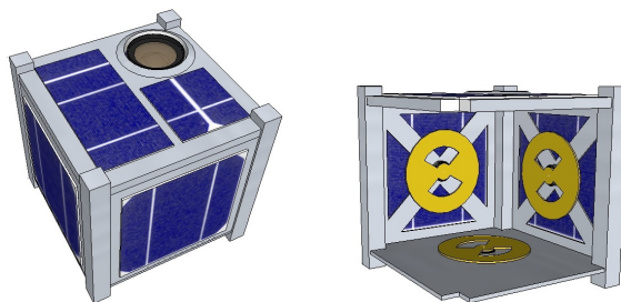
Figure 12: A spacecraft/rover hybrid is a planetary mobility platform sealed in one enclosure and actuated through three mutually orthogonal flywheels (for clarity, internal payload is not shown). By spinning the flywheels, one gives rise to surface reaction forces that make the rover tumble or hop. External spikes/feet (not shown here for clarity) are added to protect instruments and solar panels, and to improve traction. Trade-offs for spike design are discussed in Section 3.3.
