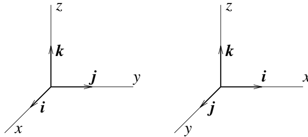
Figure 2.7: Right and left handed coordinate systems.
