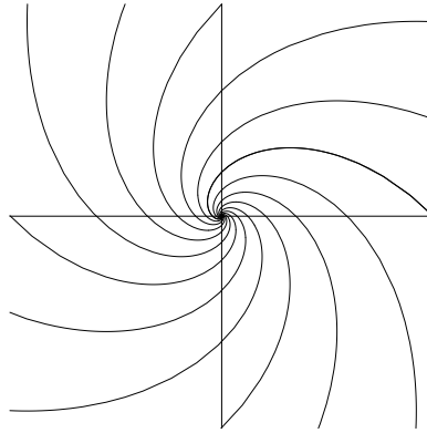
Figure 8.8: Streamlines for \psi = \ln r + \theta .
