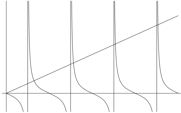
Figure 29.1: x and -\tan(x) .
