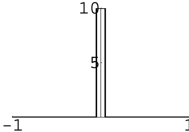
Figure 20.2: Graph of b(x, 1/10) .
