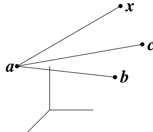
Figure 2.11: Three points define a plane.
