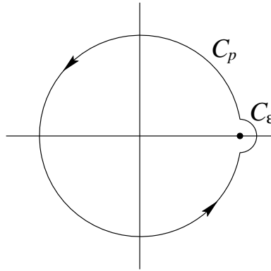
Figure 13.4: The C_\epsilon Contour
