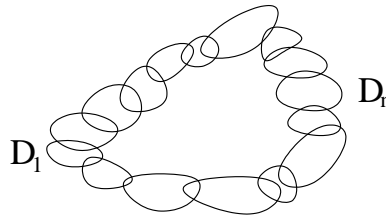
Figure 9.2: Two Paths of Analytic Continuation
