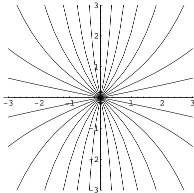
Figure 48.4: \sinh(cx)
