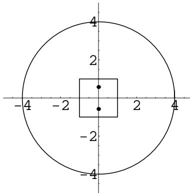
Figure 11.2: The contours and the singularities of \frac{1}{3z^2+1} .
