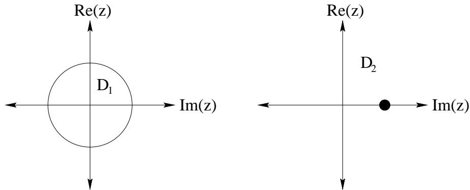
Figure 9.5: Domain of Convergence for \sum_{n=0}^{\infty} z^n .
