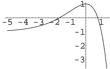
Figure 14.11: The function 2(1-x)e^x - 1 .
