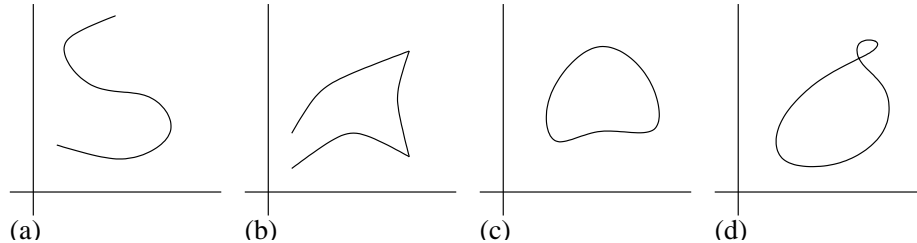
Figure 7.1: (a) Smooth curve. (b) Piecewise smooth curve. (c) Simple closed curve. (d) Non-simple closed curve.
