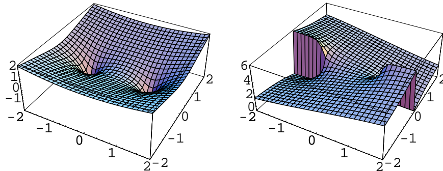
Figure 8.10: The velocity potential \phi and stream function \psi for \Phi(z) = \log(z - 1) + \log(z + 1) .
