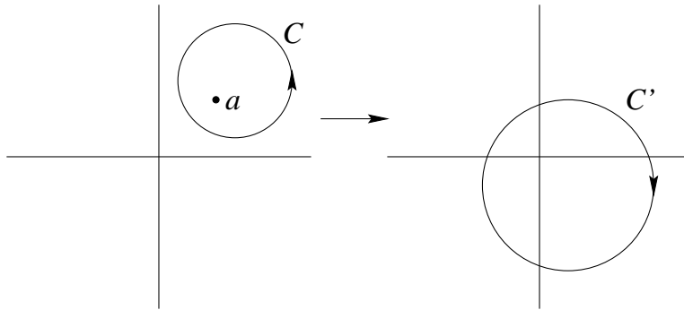
Figure 13.3: The change of variables \zeta = 1/(z - a) .
