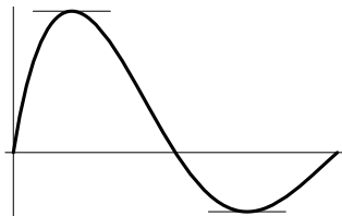
Figure 3.9: Rolle's Theorem.
