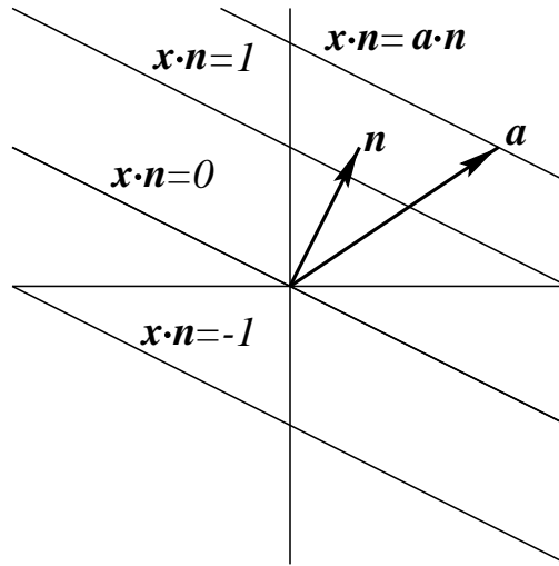
Figure 2.5: Equation for a line.
