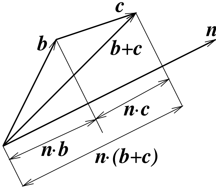
Figure 2.12: The distributive law for the dot product.
