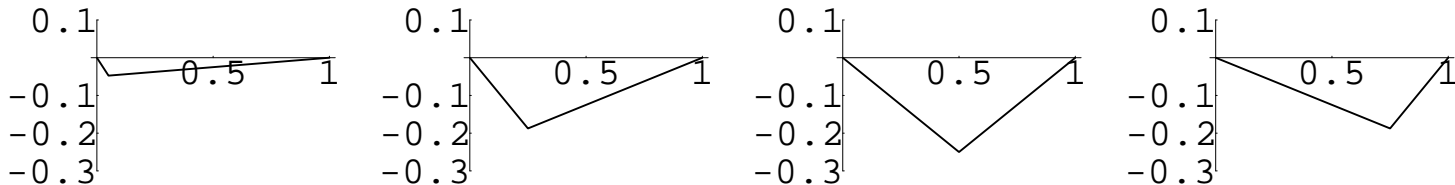
Figure 21.3: Plot of G(x|0.05), G(x|0.25), G(x|0.5) and G(x|0.75) .
