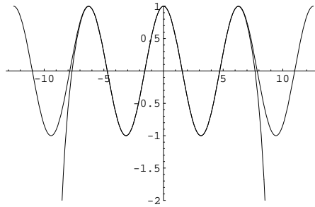
Figure 3.14: Ten Term Taylor Series Approximation of \cos x
