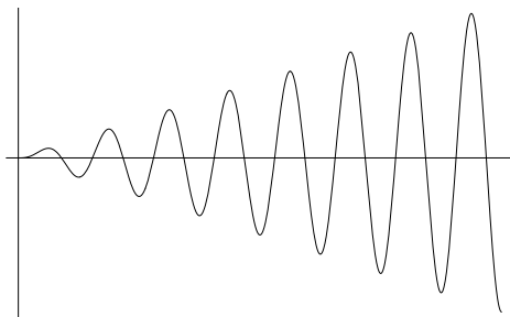
Figure 21.6: Resonant Forcing
