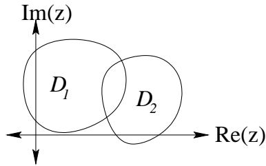
Figure 9.1: Overlapping Domains
