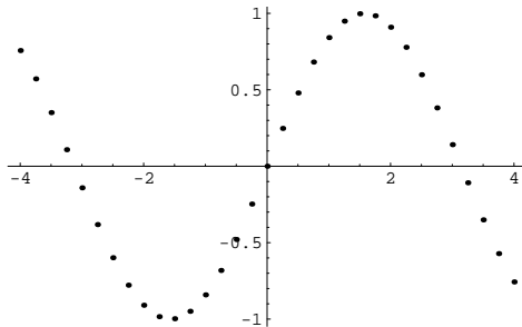
Figure 3.16: Sampling of \sin x
