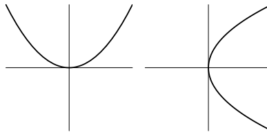
Figure 1.2: Diagrams of One-To-One, Many-To-One and One-To-Many Functions
