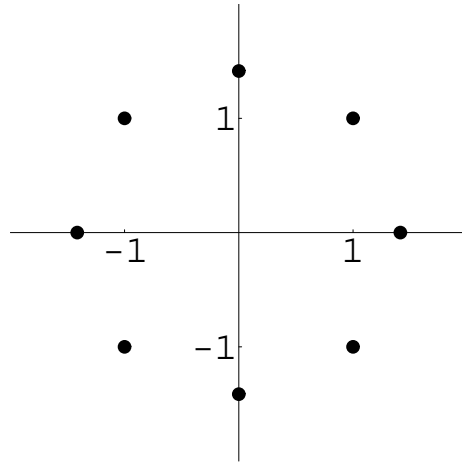
Figure 6.18: 16^{-1/8}
