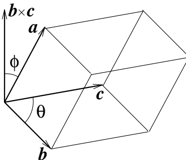
Figure 2.10: The parallelepiped defined by three vectors.
