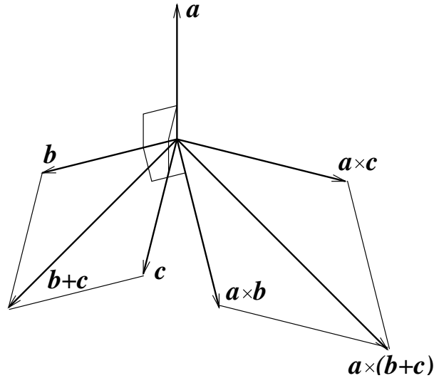
Figure 2.13: The distributive law for the cross product.
