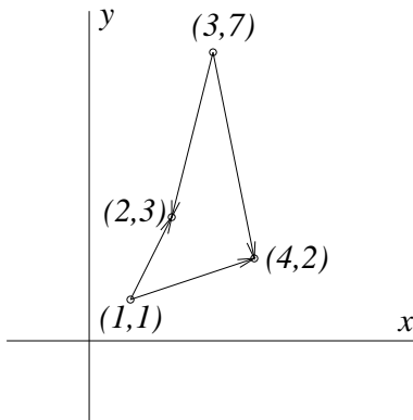
Figure 2.15: Quadrilateral.
