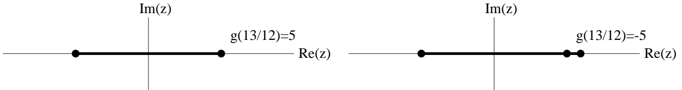
Figure 7.54: The branch cuts for f(z) = \log\left(5 + \left(\frac{z+1}{z-1}\right)^{1/2}\right) .
