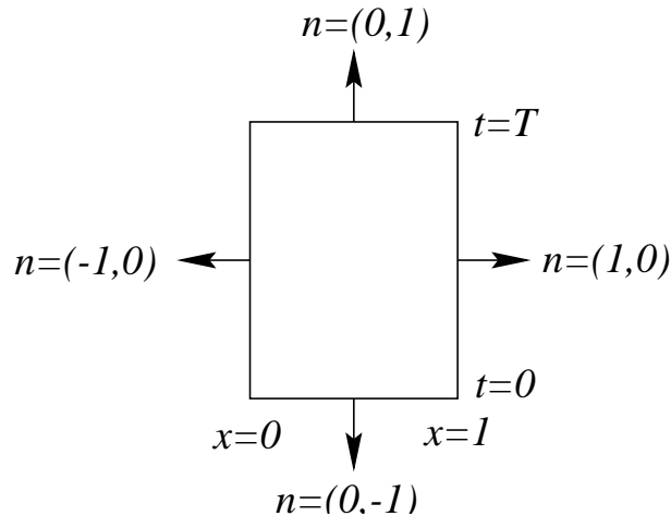
Figure 45.7: Outward normal vectors of the domain.
