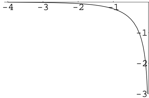
Figure 12.3: The Exponential Integral Function.
