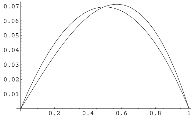
Figure 48.5: One Term Approximation and Exact Solution.
