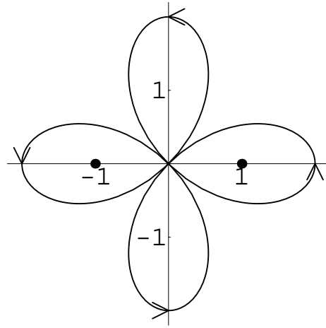
Figure 13.7: The contour r = 2 \cos(2\theta) .
