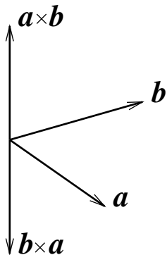
Figure 2.8: The cross product is anti-commutative.
