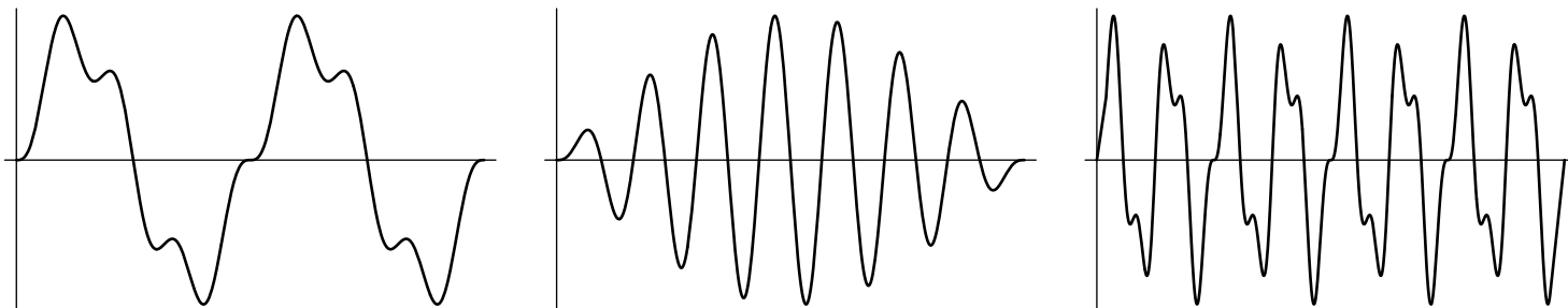
Figure 21.5: Non-resonant Forcing
