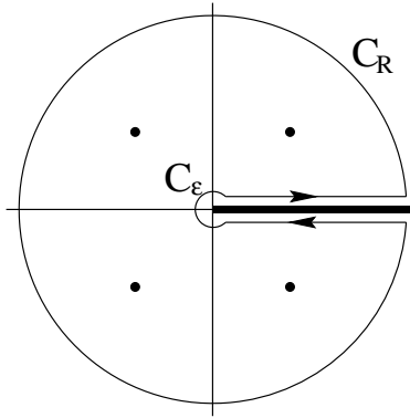
Figure 13.12: Possible path of integration for f(z) = \frac{z^a}{1+z^4}
