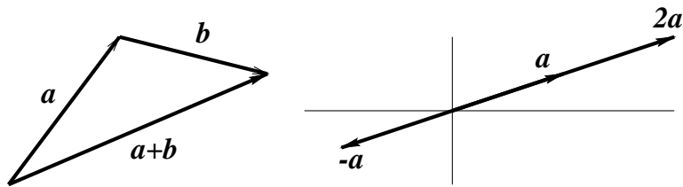
Figure 2.2: Vector arithmetic.
