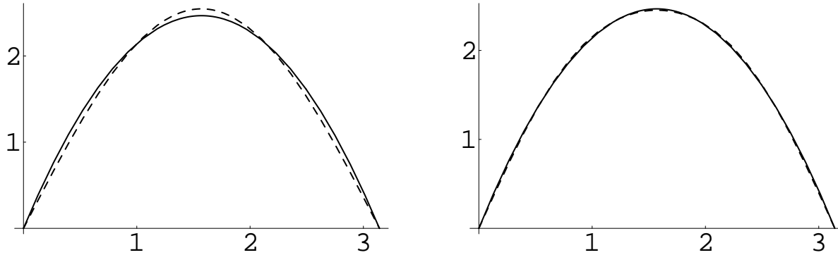
Figure 25.2: Series Expansions of x(\pi - x) .
