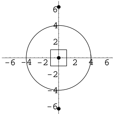
Figure 11.3: The contours and the singularities of \frac{z}{1-e^z} .
