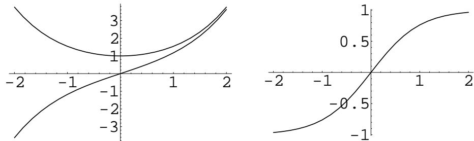
Figure M.1: \cosh x , \sinh x and then \tanh x
