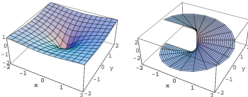
Figure 7.21: Plots of \Re(\text{Log } z) and \Im(\text{Log } z) .
