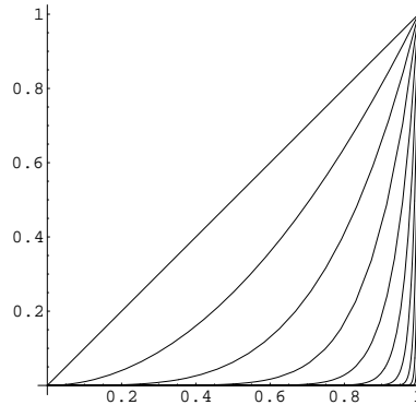
Figure 4.3: Plots of x^1, x^2, x^4, x^8, \dots, x^{1024} .
