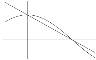
Figure 13.16: \cos(2\theta) and 1 - \frac{4}{\pi}\theta
