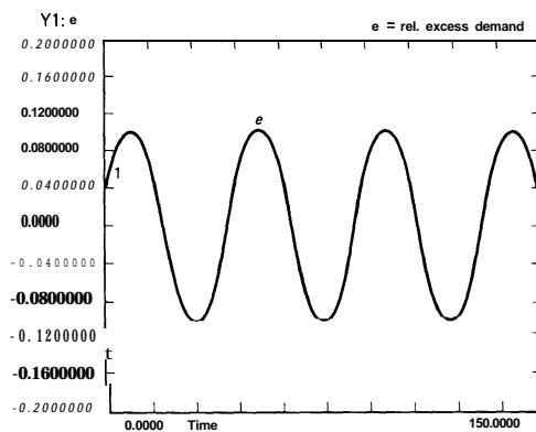
Figure 14.2 Limit cycle in e
