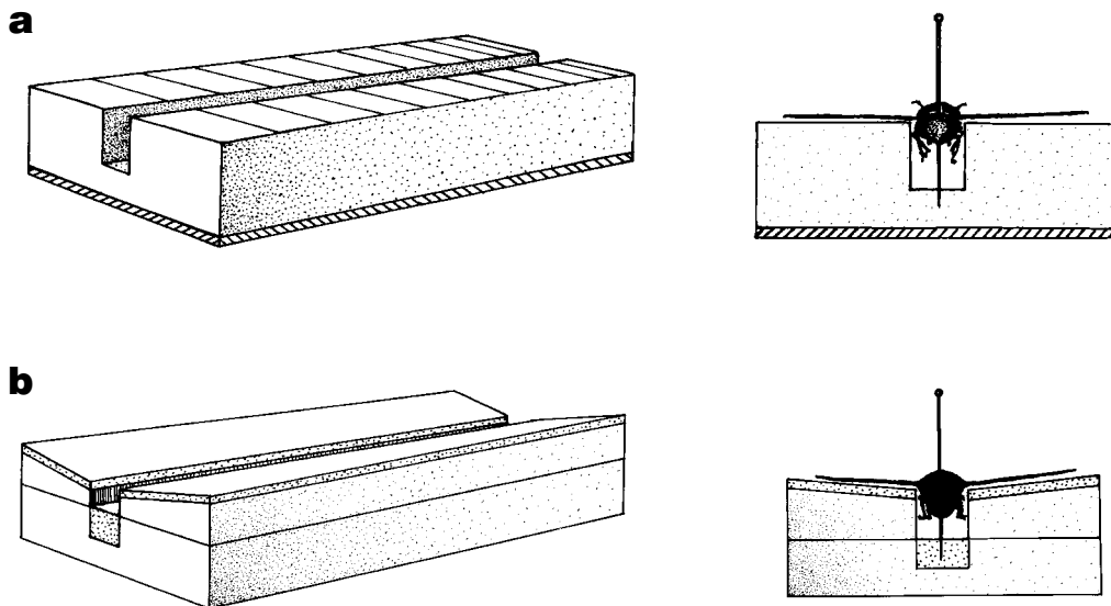
Fig. 76. (a) Standard setting board; (b) angled setting board
