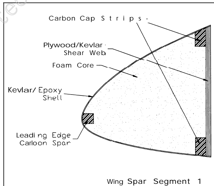
Figure 5. Cross-sectional construction of the wing spar.
