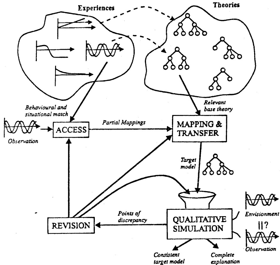
Figure 2. The architecture of PHINEAS. In PHINEAS, SME was used as a module in a system that learns qualitative models of physical phenomena via analogy. PHINEAS' map/analyse cycle is a good example of how SME can be used in systems that interleave representation construction with other operations.
