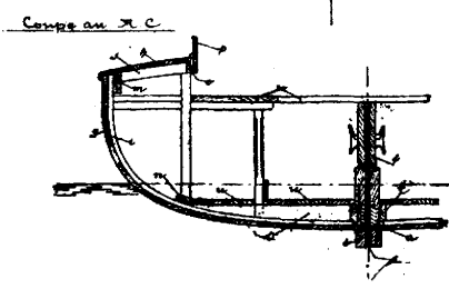
Plan de construction.
