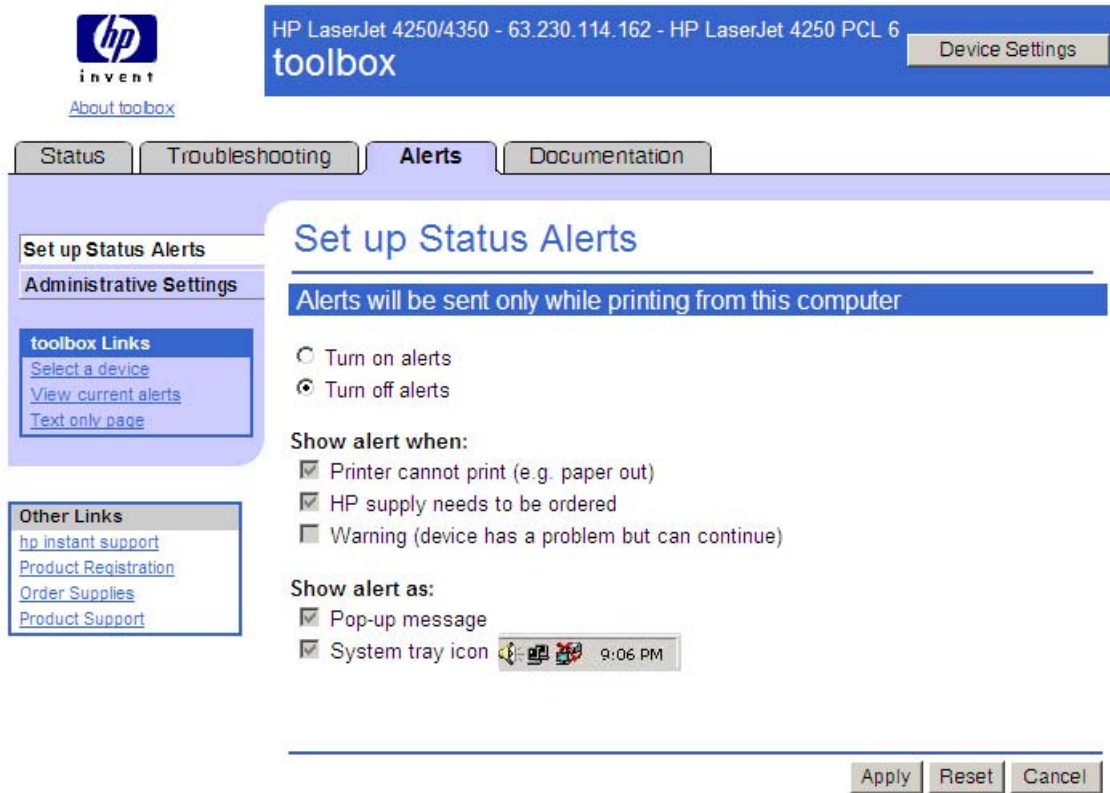
Figure 2-14 Alerts tab
