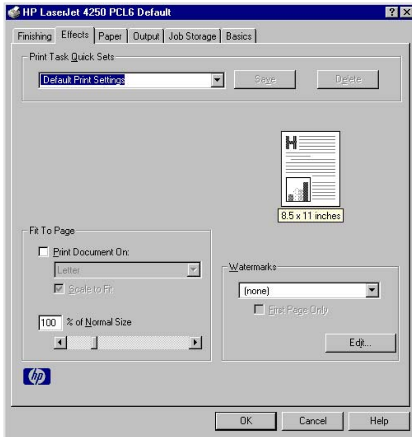
Figure 3-9 Effects tab
