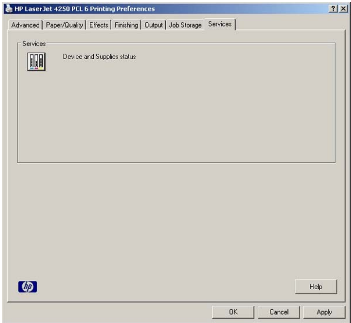
Figure 4-19 Services tab
