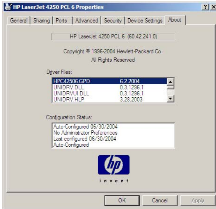
Figure 4-24 About tab
