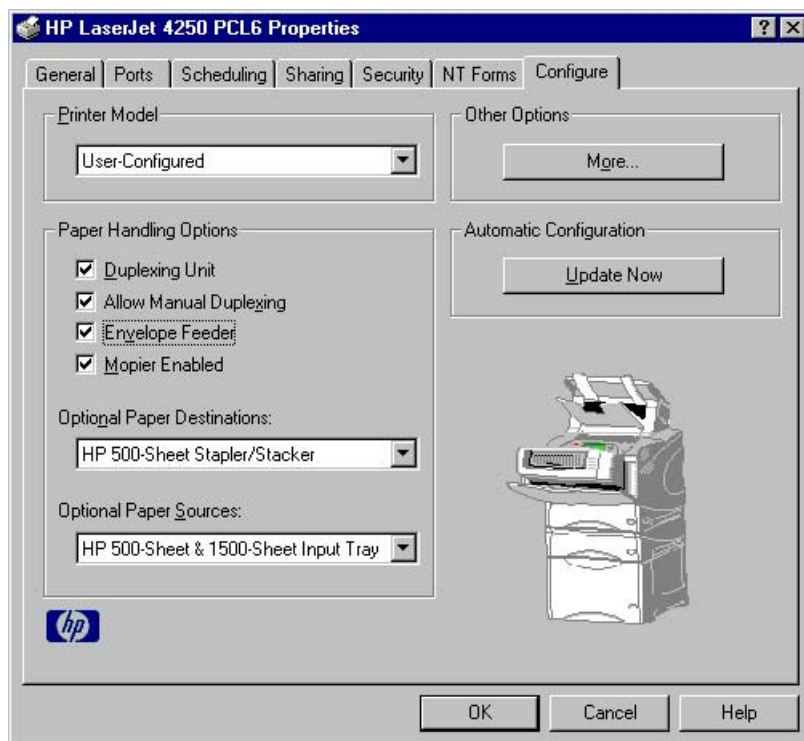
Figure 3-25 Configure tab
