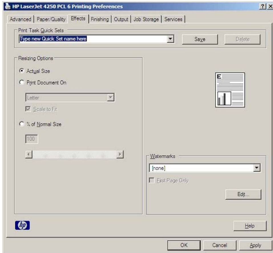
Figure 4-11 Effects tab
