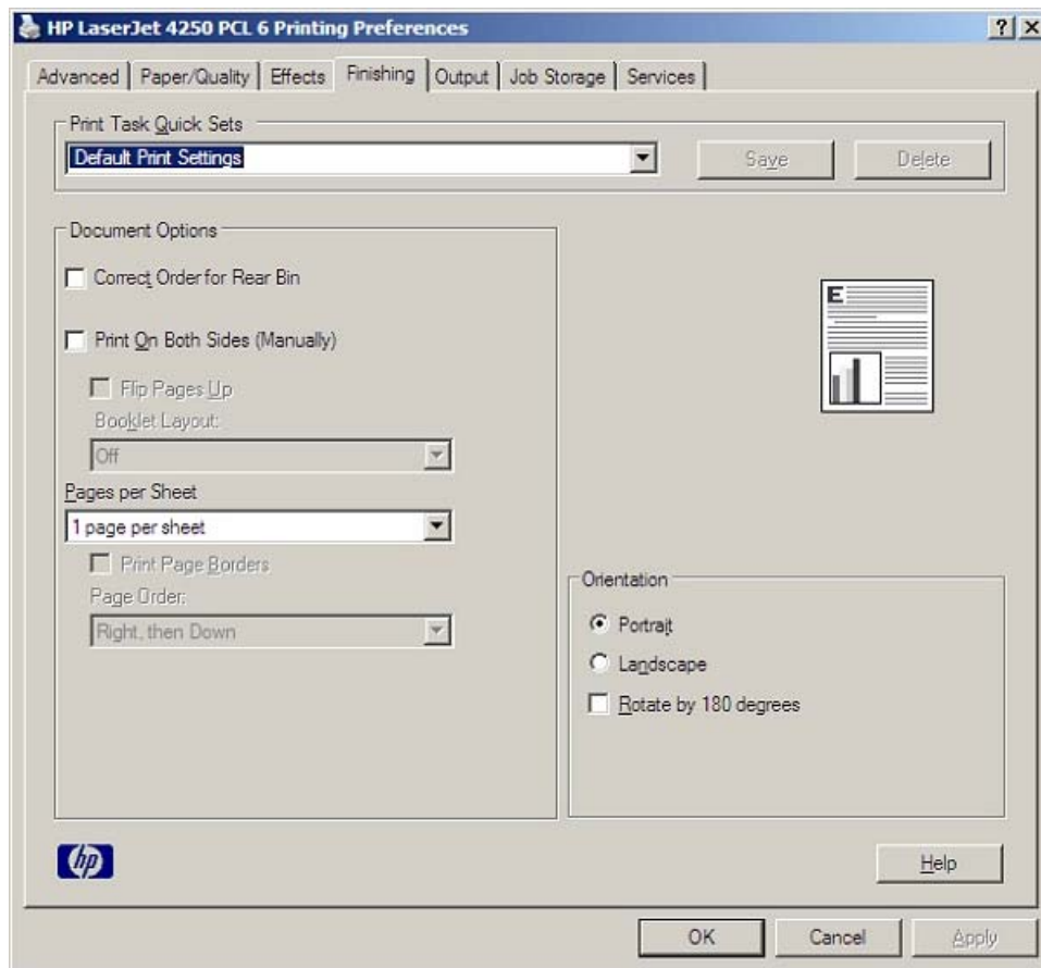
Figure 4-14 Finishing tab
