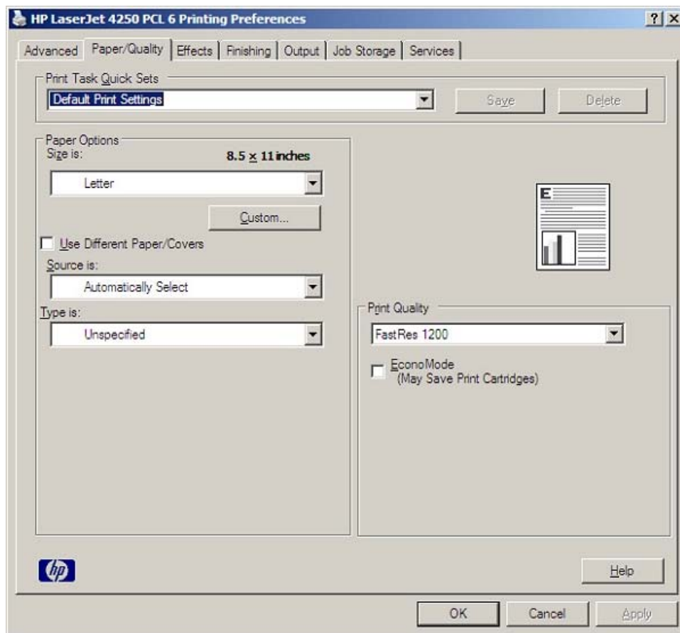
Figure 4-3 Paper/Quality tab
