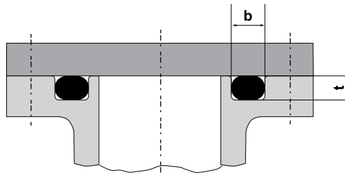
Sectional illustration of an installation space for PTFE O-rings
