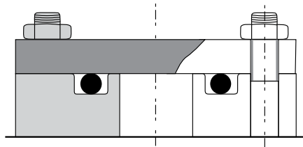
Flange seals
