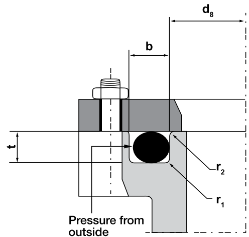
Flange seal – external pressure
