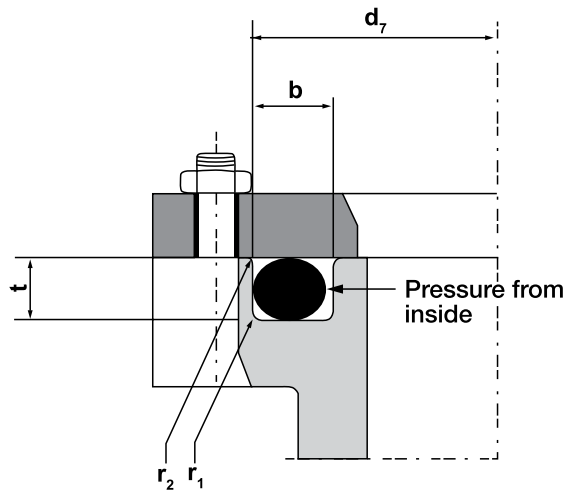
Flange seal – internal pressure
