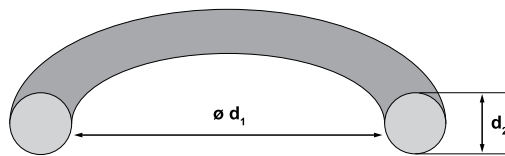
O-ring-sizing
