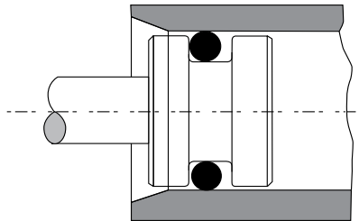
Piston seals
