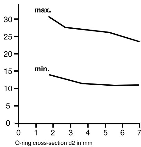
Static seal compression
