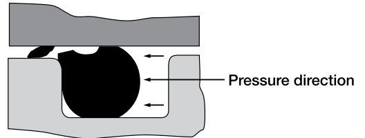
Extruded O-ring
