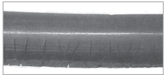
Illustration of chemical aggression on an O-ring
