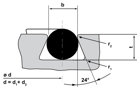
Picture of a trapezoidal groove
