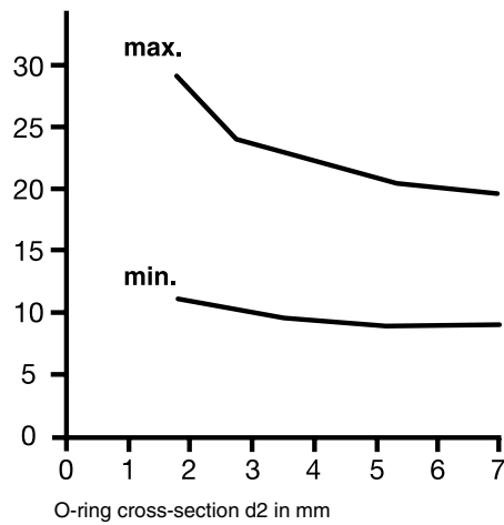
Dynamic seal compression
