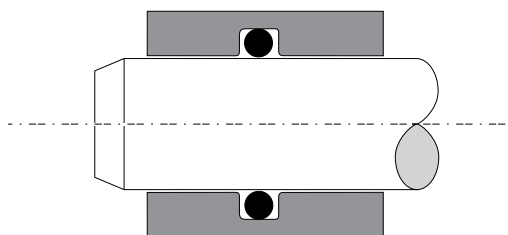
Rod seals
