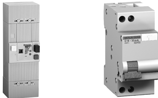
The incoming-supply circuit-breaker can also have time-delayed characteristics and integrate a RCD (type S).
