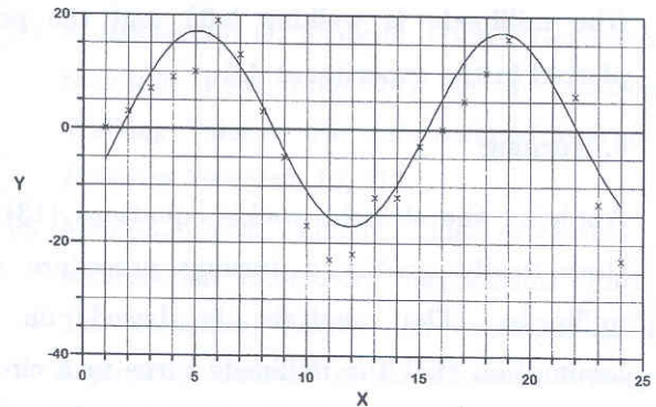
Fig. 5 A sample plot of data and the regression curve from the NLREG program
