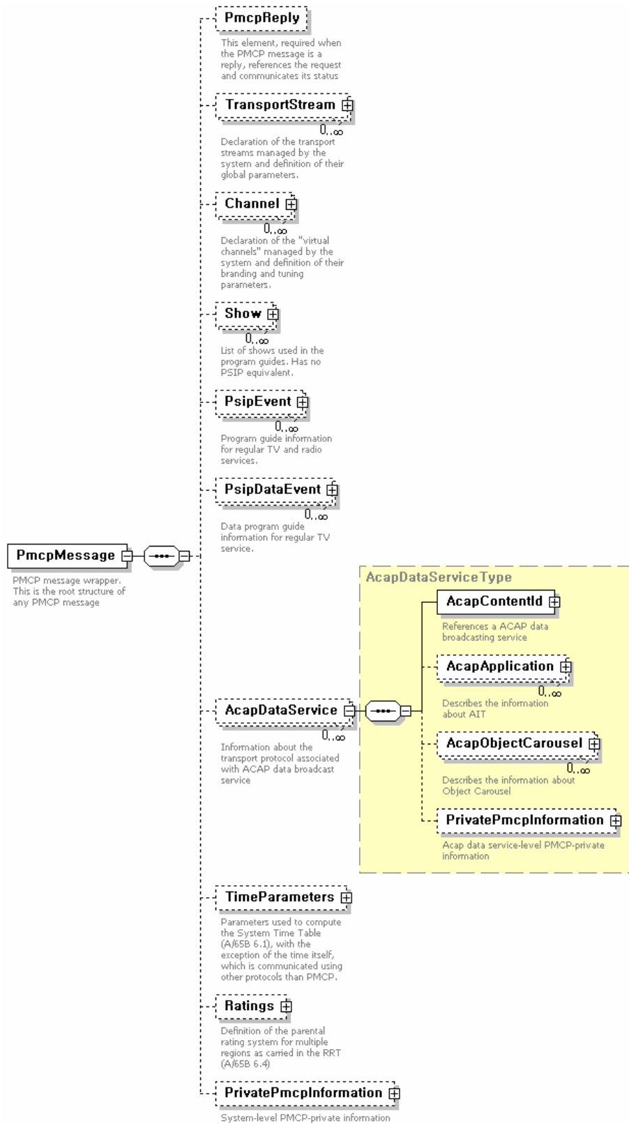
Figure D12 The Extended PMCP Schema diagram.
